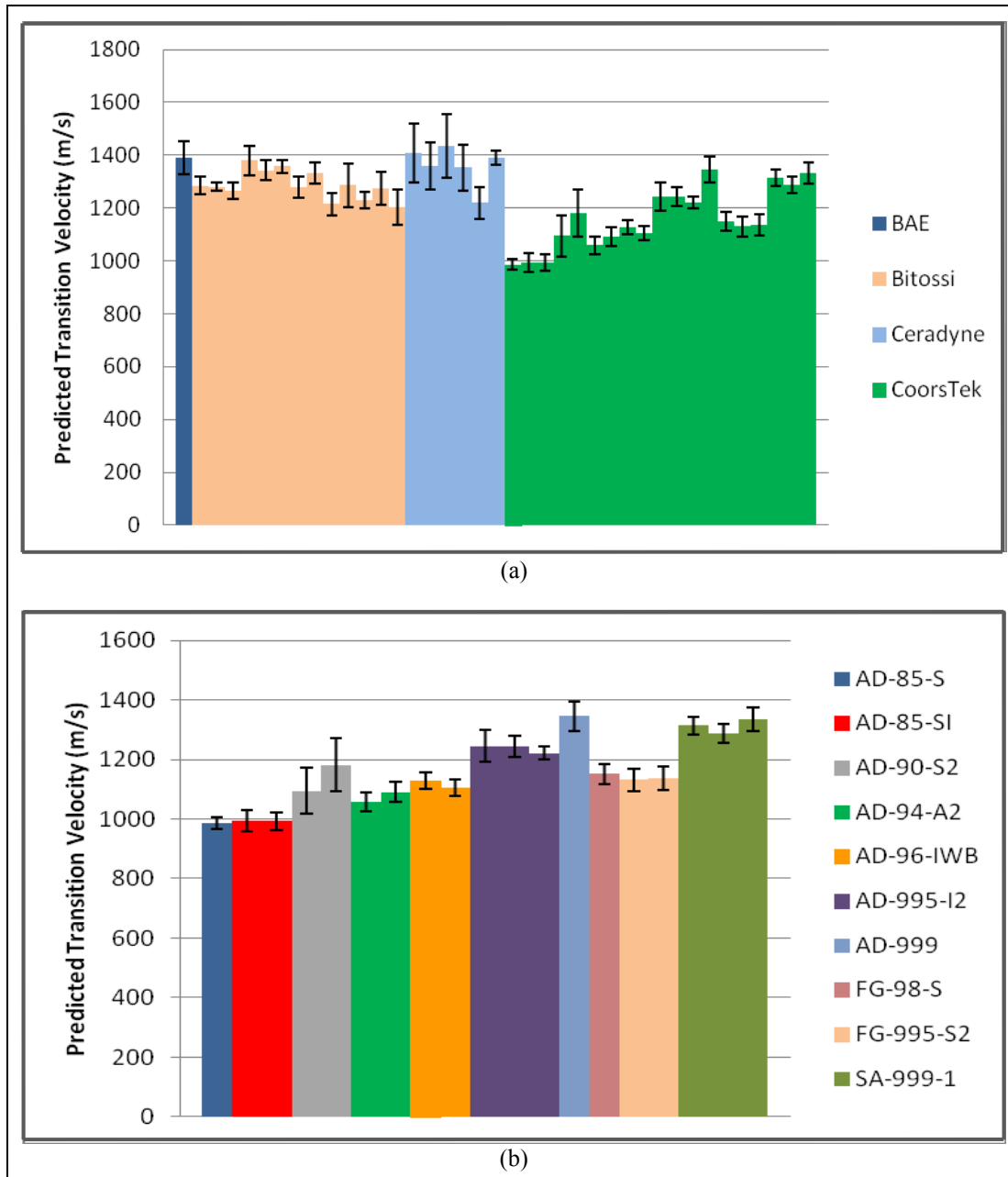
Figure 6. Predicted TVs for various \text{Al}_2\text{O}_3 materials, grouped by manufacturer (a), and predicted TVs for various CoorsTek \text{Al}_2\text{O}_3 materials (b).
