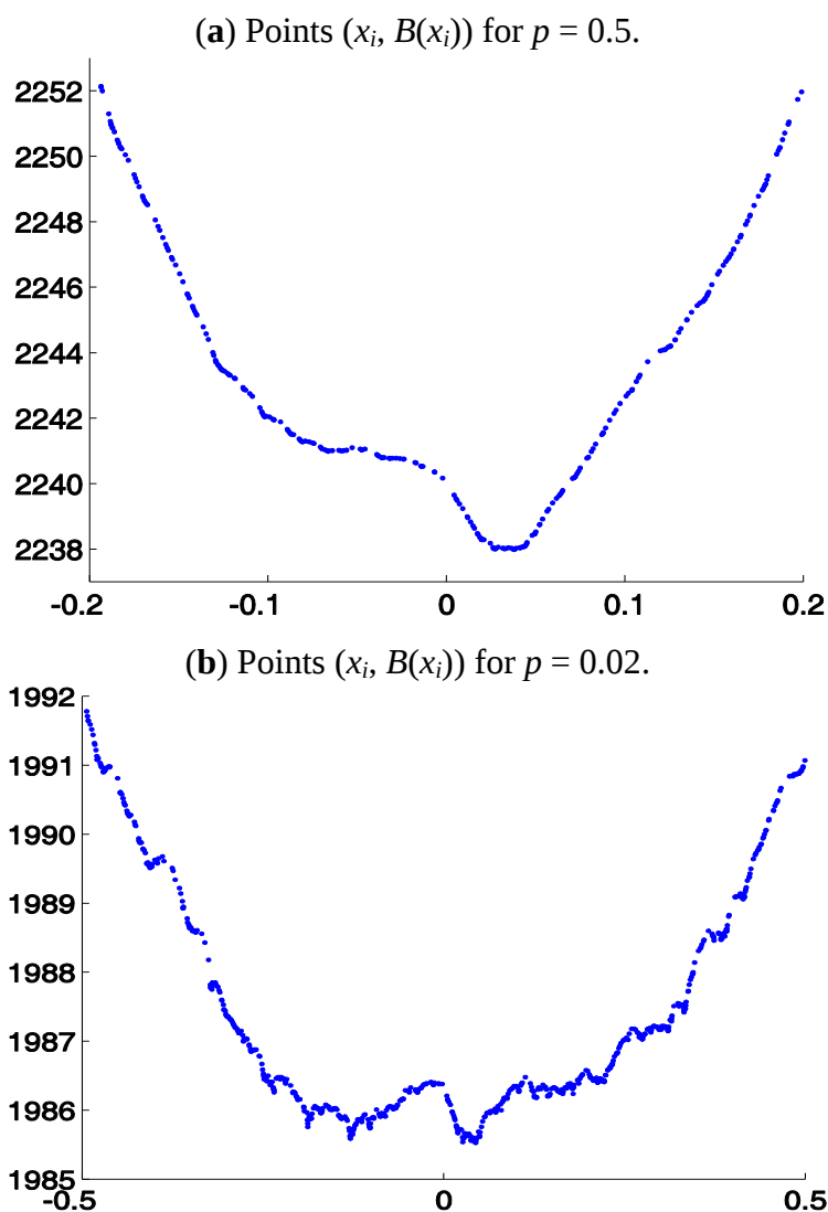
Figures 4. Points (x_i, B(x_i)) for 2000-point sample from symmetric heavy-tailed Distribution 2 with \alpha = 2 .
