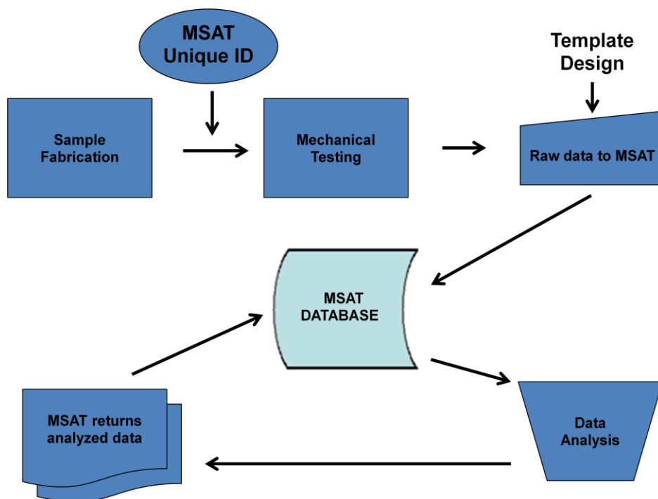
Figure 3. Work flow scheme used to transfers and converts relevant load versus displacement raw data directly to MSAT.
