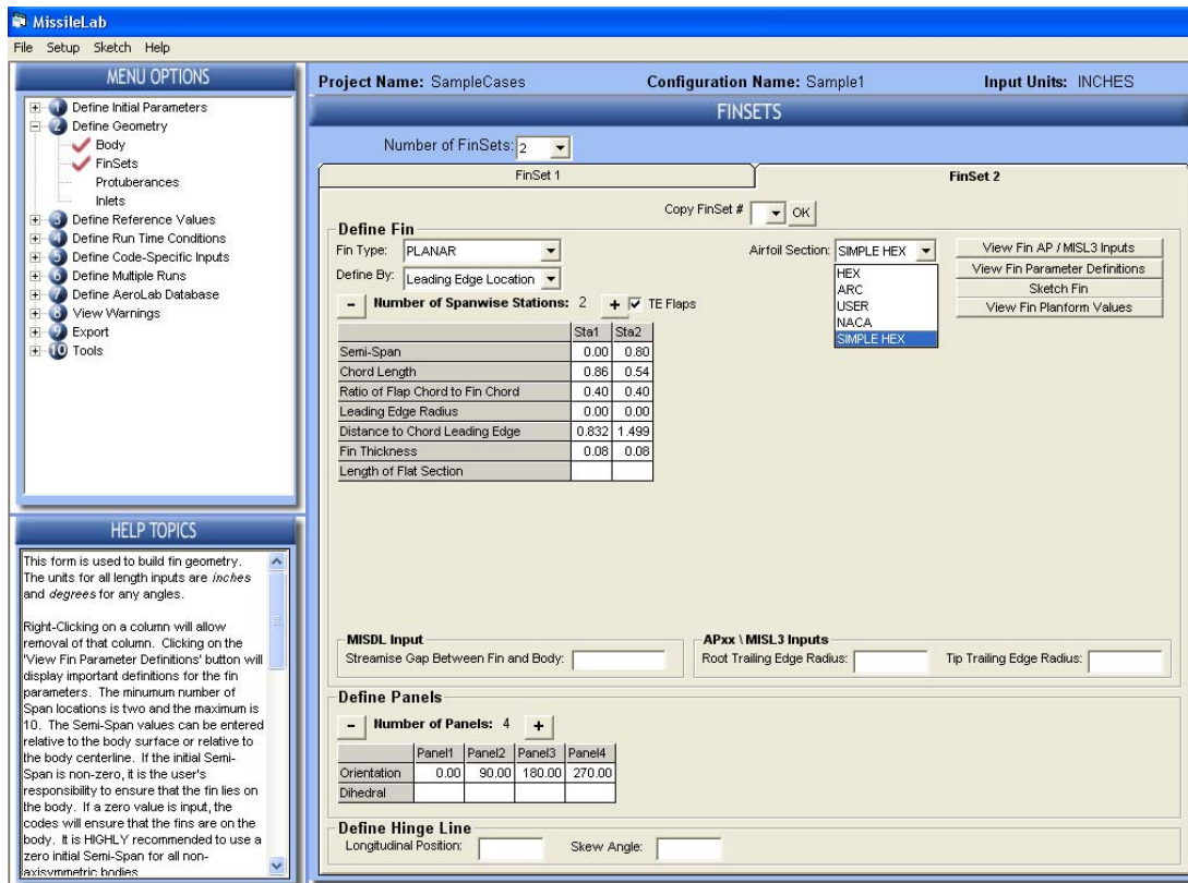
Figure 20. Fin Geometry Screen
