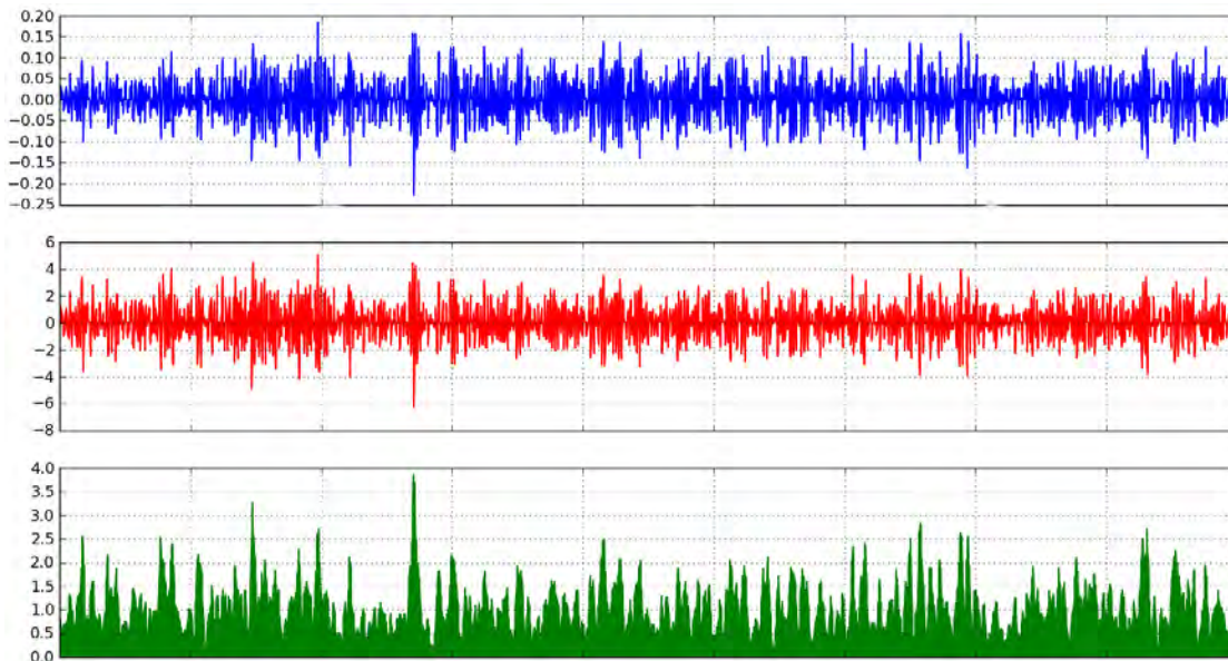
Figure 3. Same as in Figure 2 for the frequency band between 1.5 Hz and 3.0 Hz. There are two detections with SNR > 3.2 ; both are different from the two detections in Figure 2.
