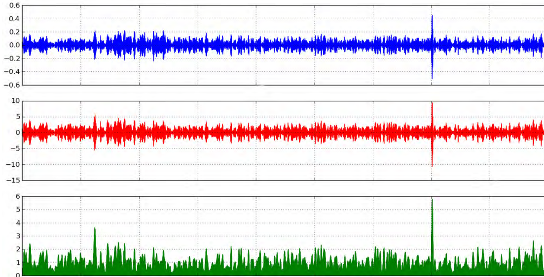
Figure 2. An example of cross-correlation analysis carried out using the template in Figure 1: blue – the normalized correlation coefficient, CC ; red – CC divided by LTA ; green – SNR = STA/LTA . The frequency band is between 2.0 Hz and 4.0 Hz. There are two detections with SNR > 3.2 .
