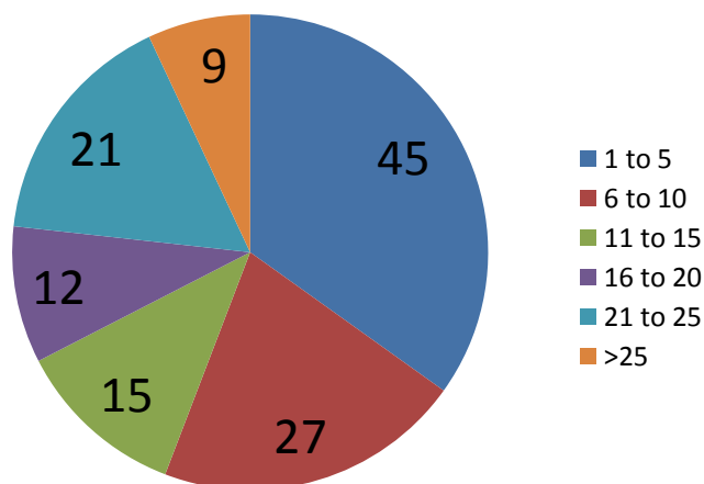
Figure 4. Distribution of the number of hits for the 129 REB events matched by cross-correlation.
