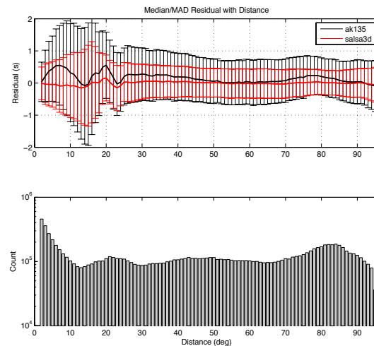
Figure 5. Travel-time residuals with distance (top) showing the median residual (solid line) and L1 spread (error bars) for residuals binned in 1° bins. Data are those used in the tomography model. The ak135 model displays significant bias, especially for regional data, while the SALSA3D reduces this bias to almost zero, with a corresponding reduction in residual spread. Bottom: counts of arrivals in each bin demonstrating about equal and adequate coverage over all distance ranges.
