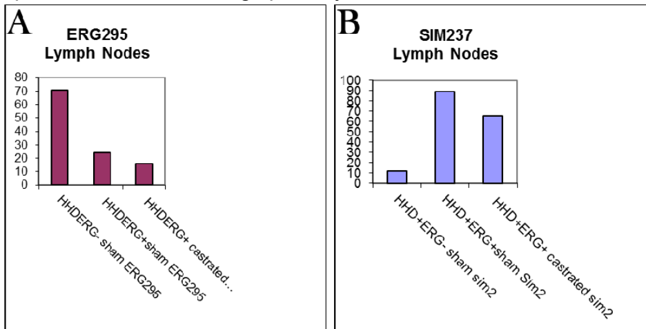
Figure 8: Effect of castration on SIM2 and ERG-specific, CTL responses. Male HHD/ERG- and HHD/ERG+ mice were surgically castrated and immunized with sim2- and ERG-derived HLA-A2.1-restricted peptides (peptides SIM237 and ERG295) 4 weeks later. IFN- \gamma ELISPOT was performed on prostate-draining lymph nodes 10 days post-immunization. Lymph nodes from 3 mice per group were pooled to obtain sufficient cells for the assay. Number of spots on the Y axis is per 10 5 cells.
