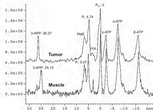
Fig. 4 31 P NMR spectra of tumor and normal muscle in presence of 3-APP. P Cr peak is the reference at 0 ppm.
