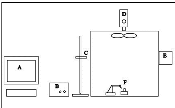
Figure 4.3: (left) Schematic illustration of experimental setup, where A =Computer/Oscilloscope, B = Electric current/ignition source, C = Detector/Sensor, D = Fan, E = Light source and F = Test-sample. (right) photo of the smoke box .
