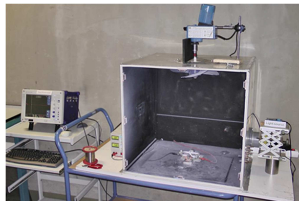
Figure 4.3: (left) Schematic illustration of experimental setup, where A =Computer/Oscilloscope, B = Electric current/ignition source, C = Detector/Sensor, D = Fan, E = Light source and F = Test-sample. (right) photo of the smoke box .
