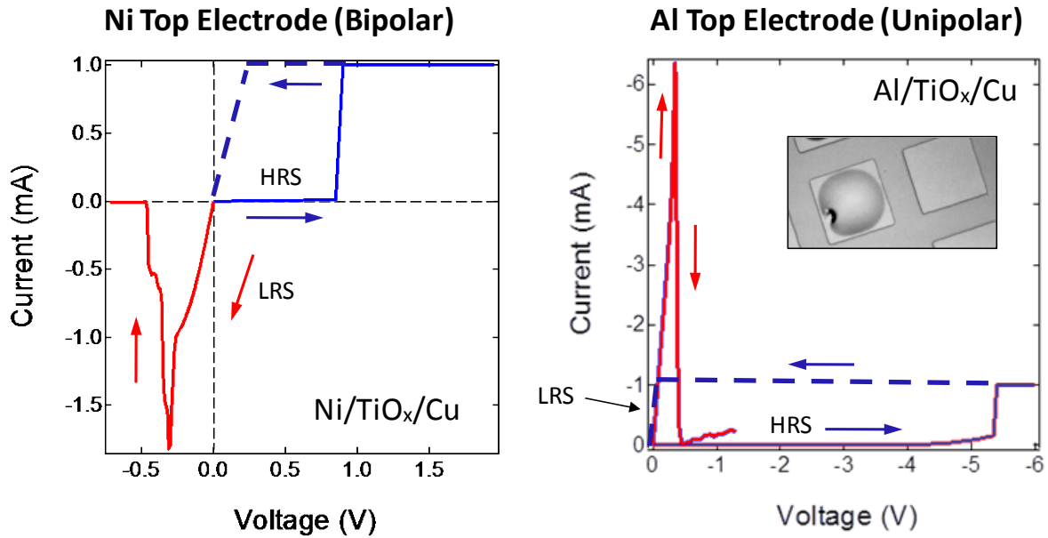
a) b) Figure 5 Current-voltage plots showing both bipolar, a), and unipolar, b), switching behavior for \text{TiO}_x devices. Bipolar behavior was observed when Ni top electrodes were used, while unipolar behavior was observed for devices with Al top electrodes. Top electrode bubbling and delamination (b), inset was observed for all \text{TiO}_x devices, regardless of top electrode material.
