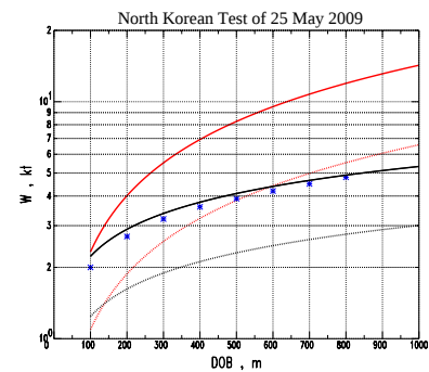
Figure 3. W:h TOCs for the 2009 NK test. Two sets are shown: black curves based on HA67 scaling and red curves for DJ91 scaling. Solid lines are \text{TOC}(M_I) s, dotted lines are \text{TOC}(m_b) . * symbols indicate TOC obtained by Murphy et al. (2010) from modeling regional P wave source spectra.
