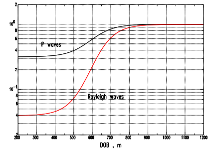
Figure 2. Coupling factors for P waves (black) and Rayleigh waves (red).
