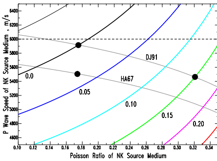
Figure 4. Contours (black dotted lines) satisfying the constraint \text{TOC}(M_I) = \text{TOC}(m_b) . Contours from equation (19) are plotted for selected \delta_{\text{NK}} ranging from -0.05 to 0.25 mu in steps of 0.05 (thin black, heavy black, blue, ..., red). A plausible upper bound on \alpha_{\text{NK}} for near-surface granite is shown by the horizontal dash line (6000 m/s).
