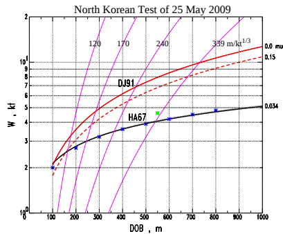
Figure 6. Revised TOCs for 2009 NK test. TOC for HA67 scaling (black) compares well with Murphy et al.'s TOC shown by * symbols on the graph, and final yield, DOB shown by * symbol. Plotted in red are “end member” solutions for DJ91 scaling with minimum and maximum \delta_{NK} (solid and dash lines). Magenta lines are for constant scaled depth of burial (e.g. 120, 169.7, 240, 339.4 m/kt 1/3 ).
