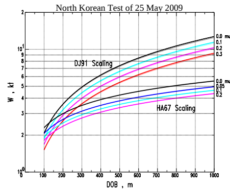
Figure 5. W:h TOCs for a range of \delta_{NK} values. TOC(M_f) and TOC(m_b) , plotted with solid and dotted lines, overlay as they should. \delta_{NK} values are: black, blue, cyan, magenta, and red for 0.0, 0.05 (HA67 only), 0.1, 0.2, and 0.3 mu (DJ91 only), respectively.
