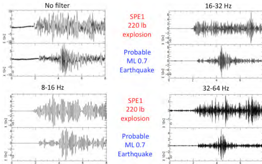
Figure 8. Comparison of SPE1 explosion and small local earthquake at similar distances.
