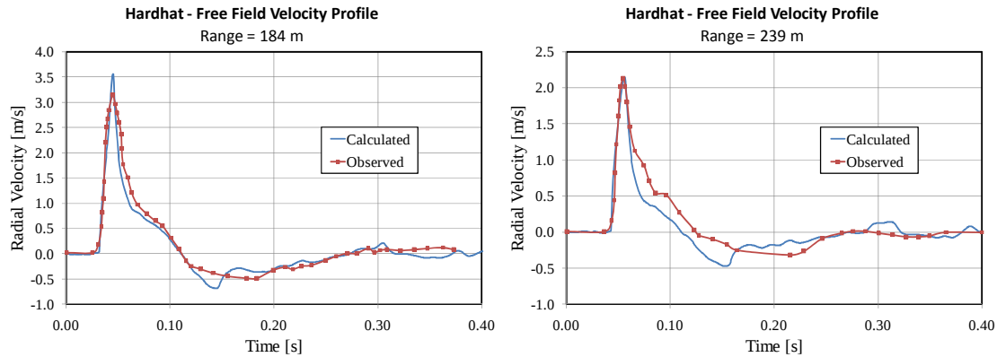
Figure 6. HARDHAT: Comparison of calculated vs. observed velocity profiles for different ranges. The calculated velocity profiles were obtained using the improved material model (with strain hardening and softening behavior).
