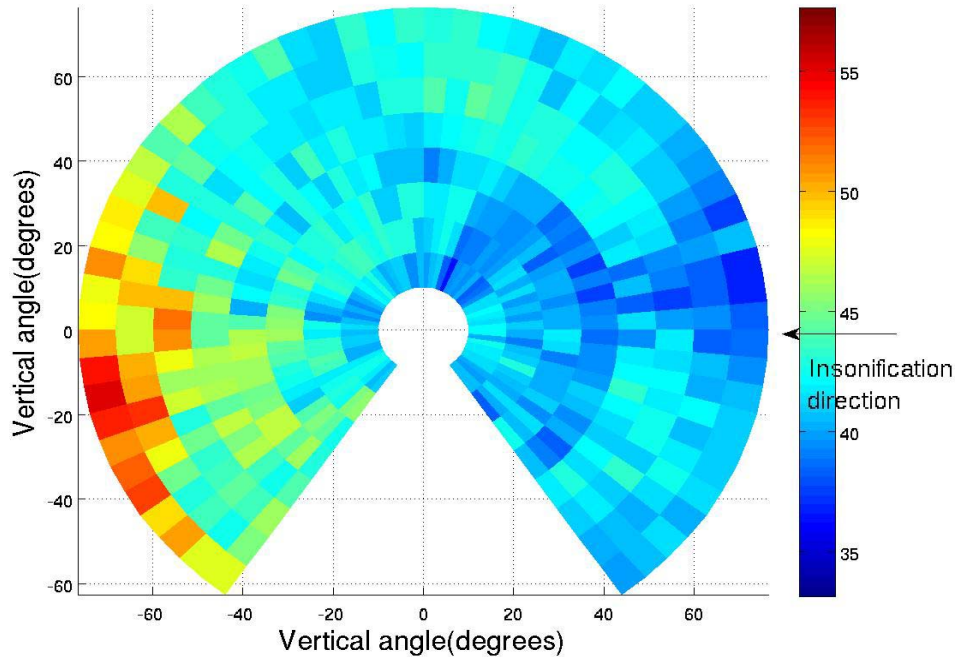
Fig. 6: Dome Mapping of average intensities in dB as a function of azimuth and vertical angles at frequency 10,000Hz
