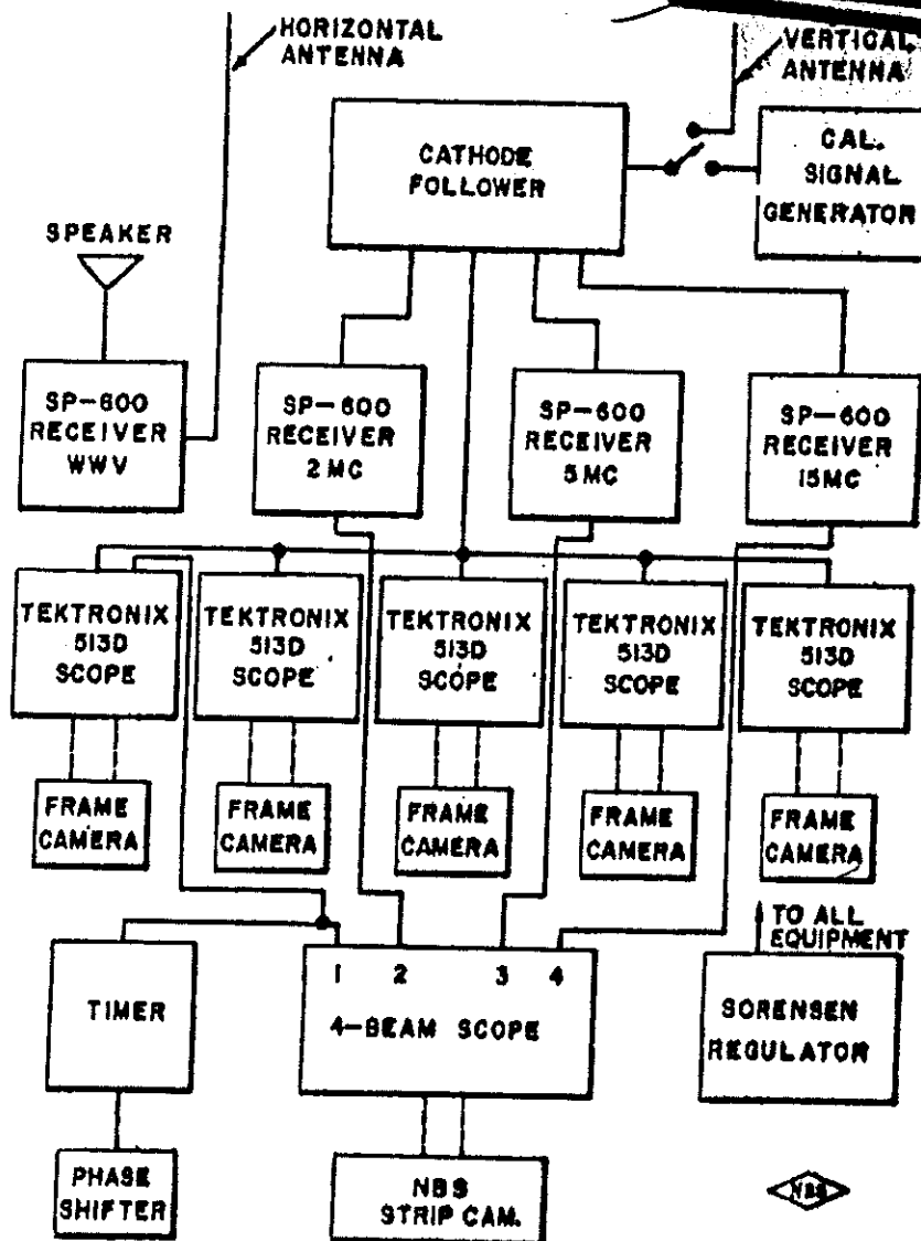
FIG. 2.1 BLOCK DIAGRAM OF EQUIPMENT USED AT THE NEVADA PROVING GROUND (MAIN SITE)
