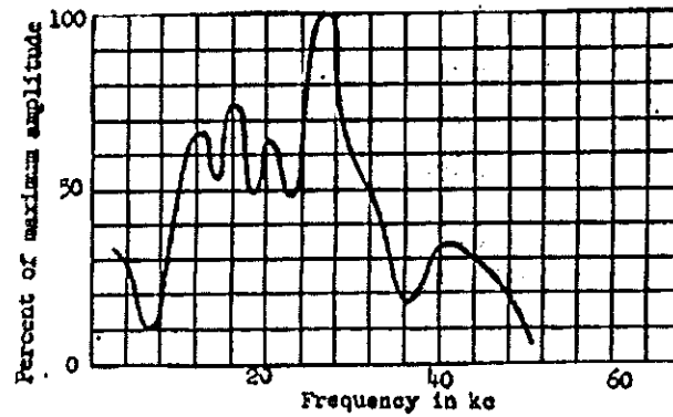
Fig. 3.63 Frequency function of broadband pulse Shot No. 2 1000 km from ground zero
