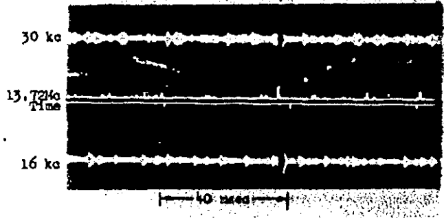
Fig. 3.95 Narrow-band responses Shot No. 4 3400 km from ground zero
