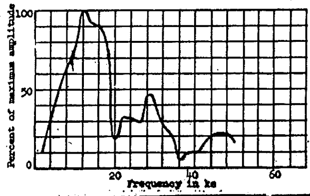
Fig. 3.76 Frequency function of broadband pulse Shot No. 6 1000 km from ground zero
