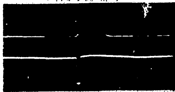
Fig. 3.77 Time comparison of second, marks from WWV (top) and timer unit Shot No. 6 1000 km from ground zero
