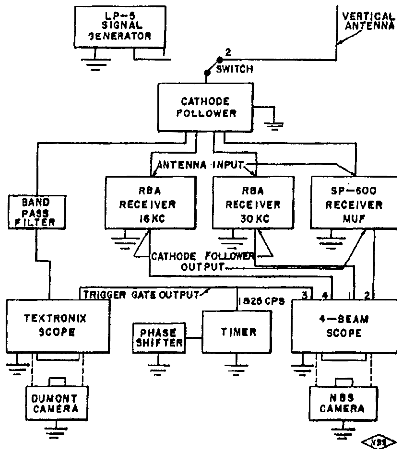
FIG. 2.6 BLOCK DIAGRAM OF EQUIPMENT USED AT BOULDER, COLO.
