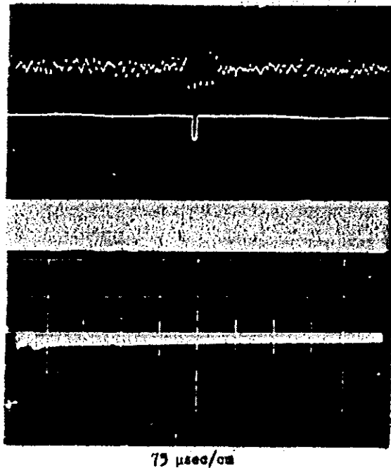
Fig. 3.65 Broadband pulse Shot No. 3 1000 km from ground zero
