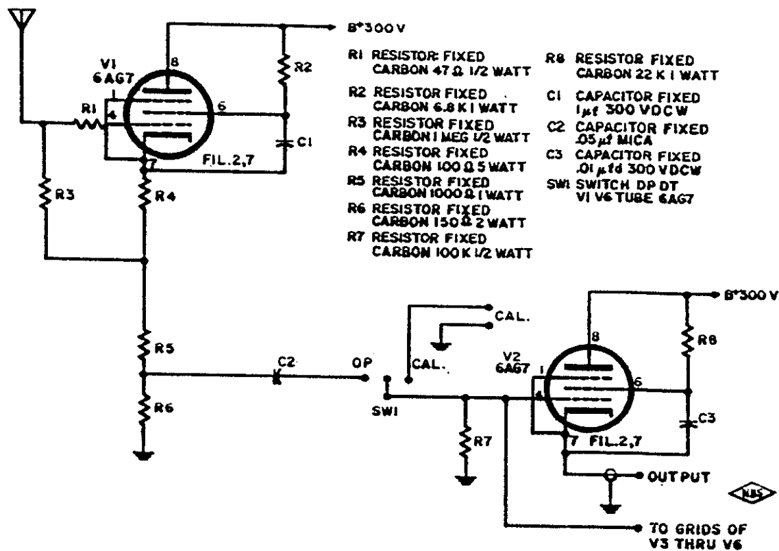
FIG. 2.2 CATHODE FOLLOWER UNIT USED AT THE NEVADA PROVING GROUND (MAIN SITE) FOR SHOT NO. 2
