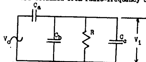
Antenna Equivalent Circuit Washington, D. C.
