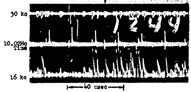
Fig. 3.96 Narrow-band responses Shot No. 5 3400 km from ground zero
