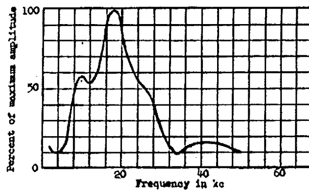
Frequency function of broadband pulse Shot No. 8 1000 km from ground zero
