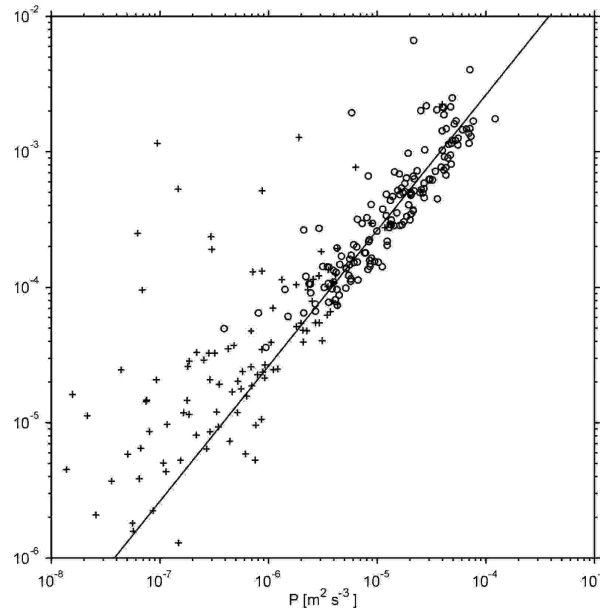
Figure 3. The rate of dissipation of TKE predicted by the closure model of Mellor and Yamada, q^3/l_m (vertical axis) versus the rate of production of TKE (horizontal axis) deduced from measurements with an ADCP in a tidal channel
