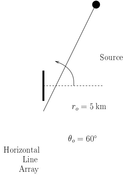
Figure 1: Top view of the geometry for the single source localization example. The source is at 60^\circ from the broadside of the horizontal receiving array, and at 5-km range.
