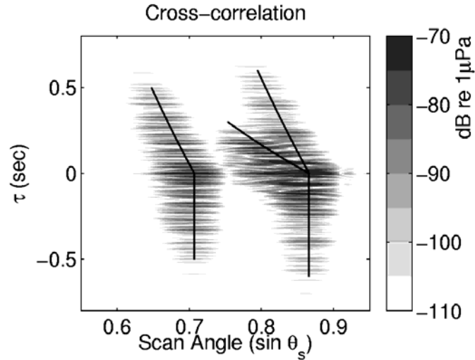
Figure 5: The cross-correlated intensity field IBo(s, \tau) for the source-receiver geometry shown in Fig. 4. The two black solid lines overlain in the \tau < 0 domain marks \sin\theta and \sin\theta_s , respectively. The three black solid lines in the \tau > 0 domain are the beamformer migration lines for sources S_1 , S_2 , and S_3 in terms of the reduced travel time.
