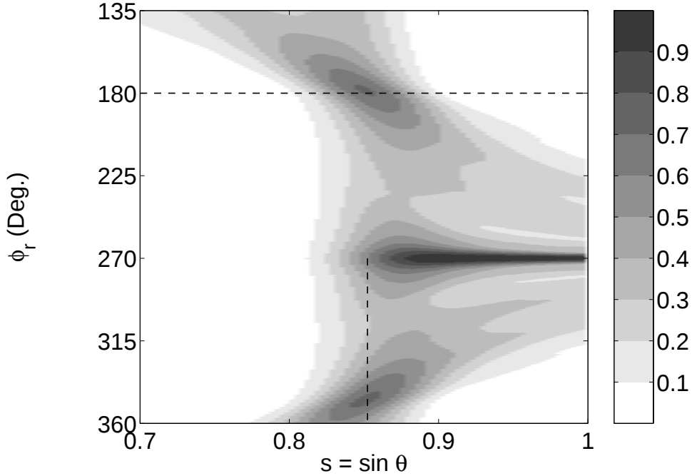
Figure 3: The transformed intensity image In(s, \phi_r) of the cross-correlated intensity image in Fig. 2.
