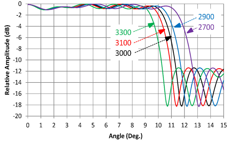
Fig. 18 — \pm 10^\circ flat-top main-beam characteristics for the linear array of 50 elements spaced \lambda/2 apart at 10 cm (3000 MHz). Element phase shifters are assumed wideband; only equivalent frequency-dependent inter-element spacing is considered.
