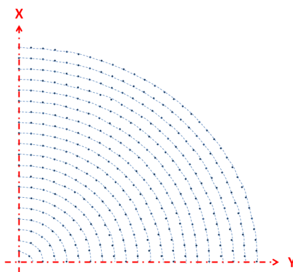
Fig. 38 — One quadrant of a concentric array grid. Elements are located in circular rings \lambda/2 apart and approximately \lambda/2 apart within each ring. 1299 elements fill a 20-ring array.
