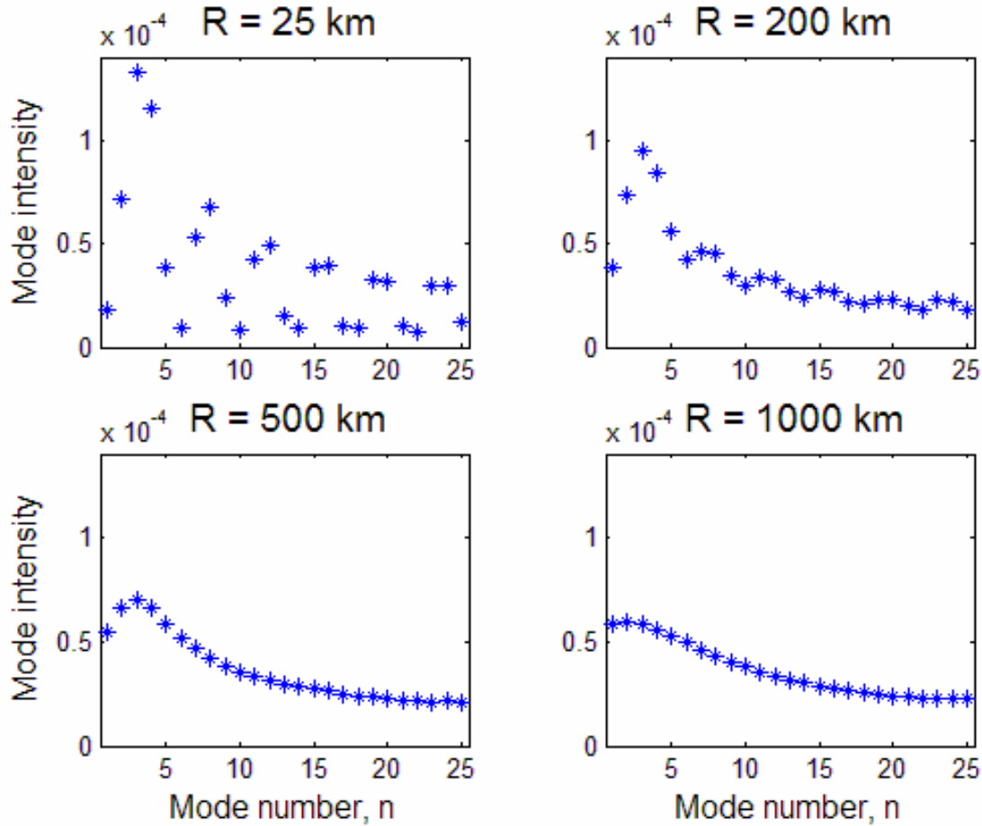
Figure 2. Mode intensities I_{nn} versus the mode number n for different propagation ranges R .
