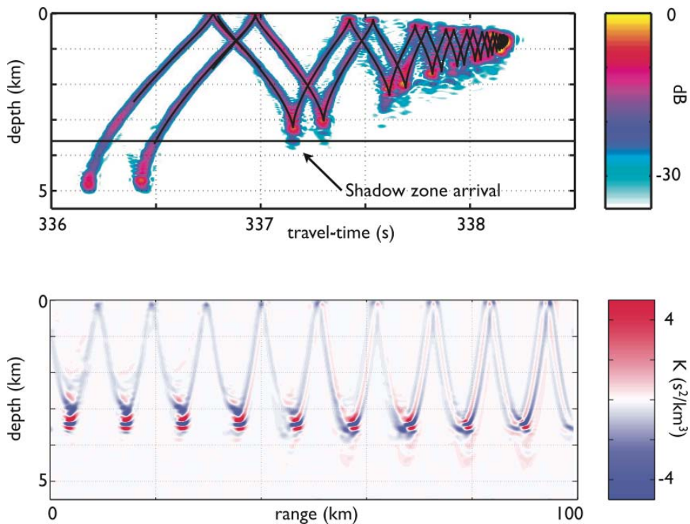
Fig. 2. (Top) The time front at 500 km range for a 75-Hz, Q=4 source at 750 m depth computed using the parabolic equation propagation code with the Garrett-Munk internal wave spectrum. The black line shows the time front in the geometric optics approximation without internal waves. (Bottom) The sensitivity as a function of range and depth of the travel time of a resolved shadow-zone arrival for a receiver at 3500 m depth that changes in sound speed. Only the first 100 km of the path is shown. Alternating blue and red colors show zones of negative and positive sensitivity with negative sensitivity along the ray path as expected.
