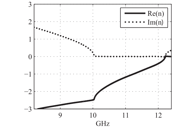
FIG. 2. Real and imaginary parts of the S-ring's retrieved refractive index. The imaginary part is near zero between 10 and 12 GHz, while the real part is negative.
