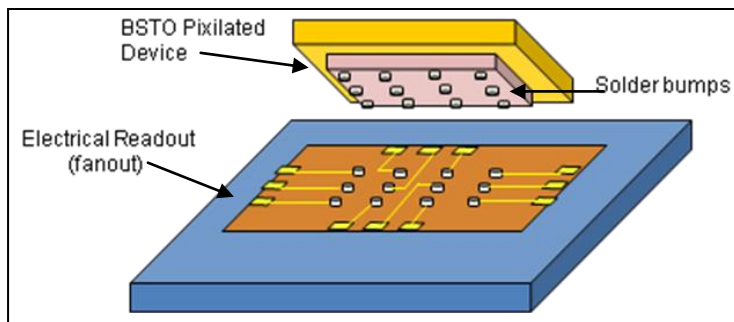
Figure 9. Diagram of hybridization between BSTO device array and silicon readout.
