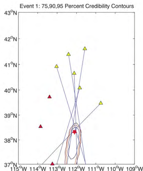
Figure 5. Location solution of epicentral infrasound estimated using the BISL method (Modrak et al., 2010). Six arrays (yellow triangles) were used in the final solution. Epicentral infrasound was not detected at the other three arrays (red triangles). The 75, 90, and 95 percent location credibility contours are shown. The seismic location is represented by the red star.
