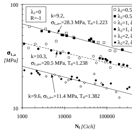
Figure 2: Influence of \lambda_2 and phase \delta on the strength of glass/polyester tubular specimen from ref.[1]).
