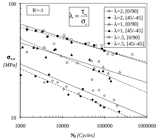
Figure 1: Off-axis angle influence on glass/polyester tubular specimen (data from ref.[1]).
