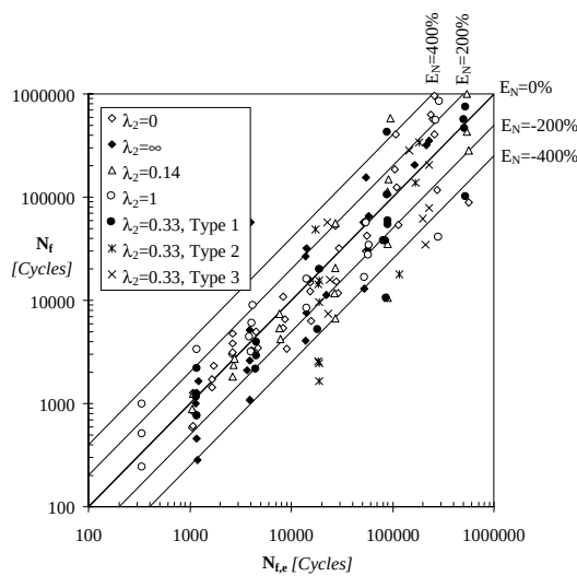
Figure 3: Estimated (Tsai-Hill) criterion experimental fatigue life [0]_N glass/polyester tubes [4].
