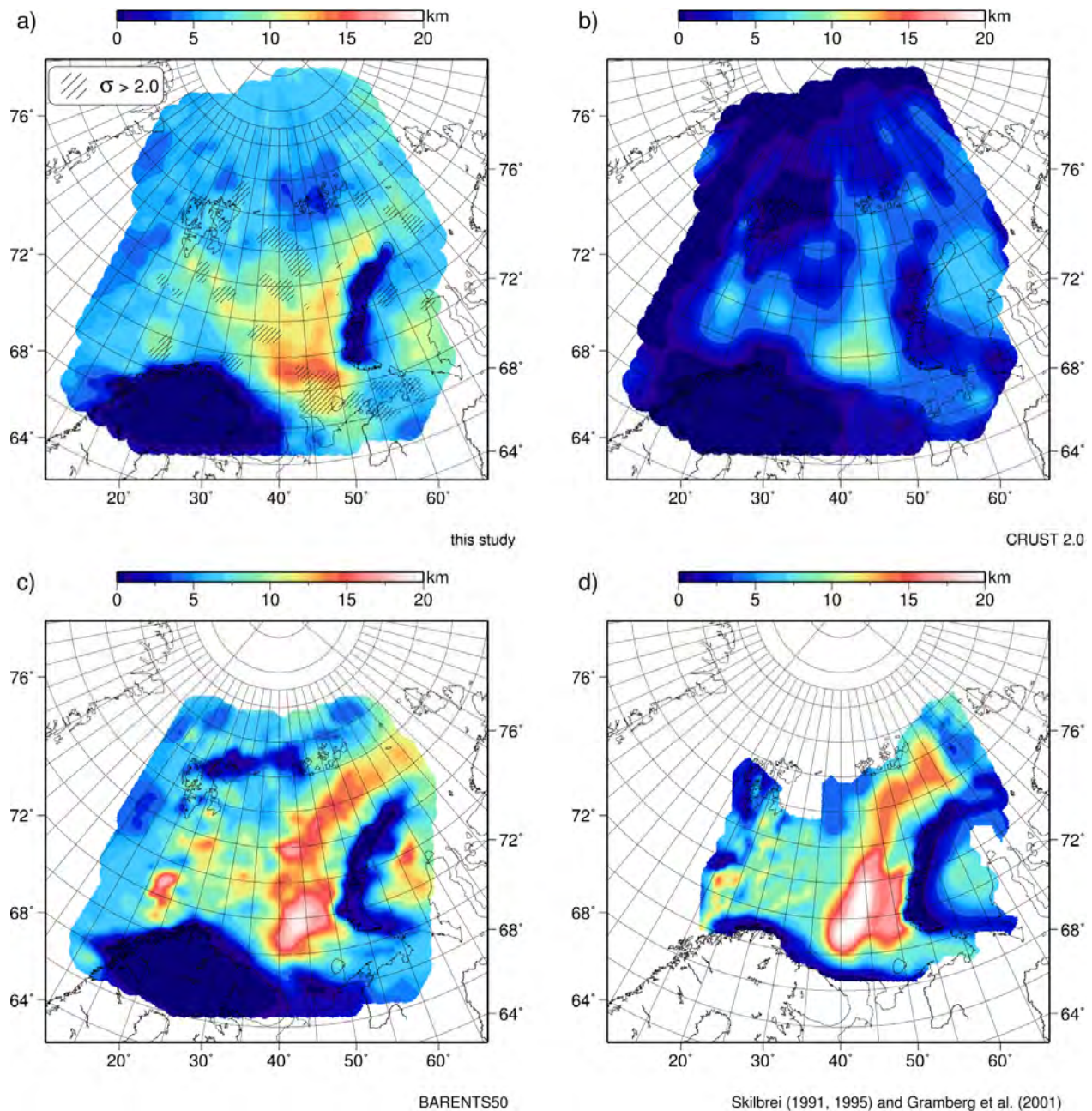
Figure 5. Depth to basement: (a) Mean model obtained in this study, (b) CRUST 2.0 after Bassin et al. (2000), (c) BARENTS50 after Ritzmann et al. (2007), and (d) compilation of depth to basement by Smelror et al. (2009), based on the work by Skilbrei (1991,1995) and Gramberg et al. (2001).
