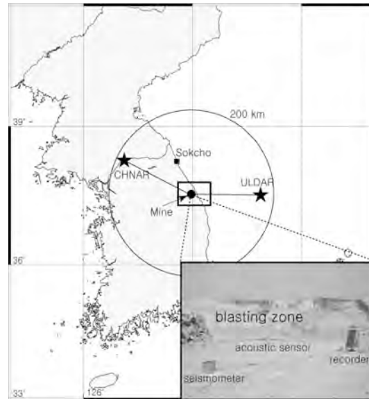
Figure 4. Locations of the open-pit mine (circle), two infrasound arrays (stars) and weather balloon station (square) used in this study. A photograph of one in-mine seismo-acoustic station is shown in the lower right.
