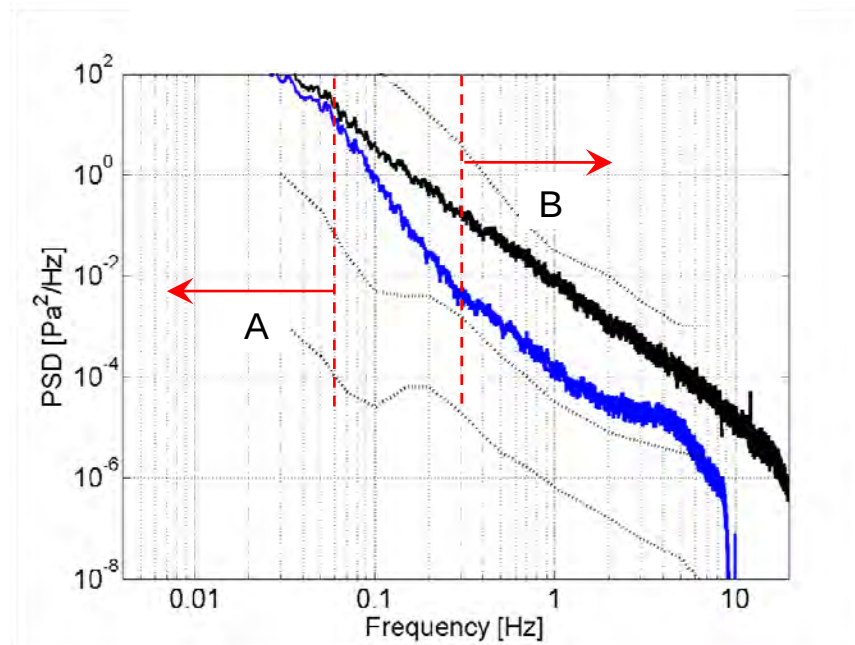
Figure 15. Pressure spectral densities for the small rosette (blue) and for the co-located reference microphone (black) for the same windy period as for Figures 13 and 14. Below 0.06 Hz (A), the spectra are nearly identical; from 0.3 to 2 Hz (B), the spectra are parallel.
