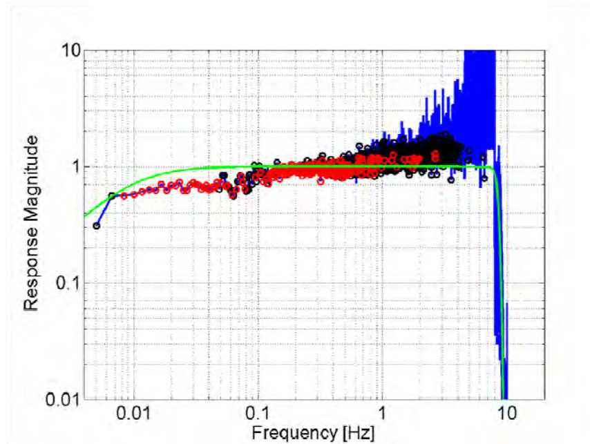
Figure 8. Magnitude response calculation for the large rosette element (V1-BFL). The calculation represents a 50-minute period starting at Day 145 01:42 UTC. The reference channel is Microphone 4. An apparent offset in magnitude response, similar to that for the large hexagonal element, appears in the 0.008 to 0.08 Hz range.
