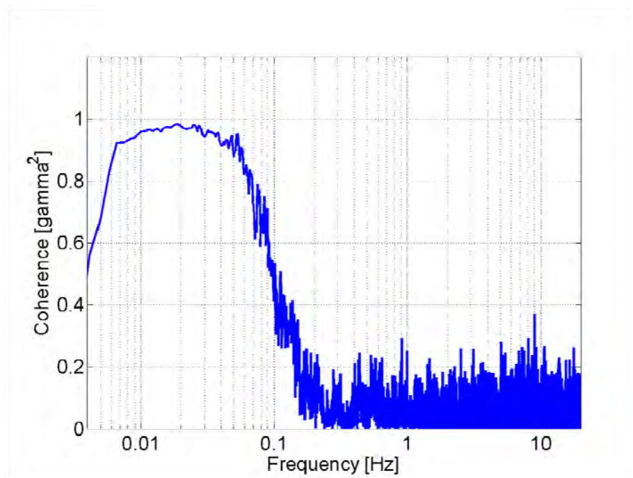
Figure 13. Coherence between the co-located reference microphone (Microphone 4) and the small rosette (V1-BFH) during a period of moderate wind. The coherence is still high below 0.07 Hz but is very low above 0.1 Hz.
