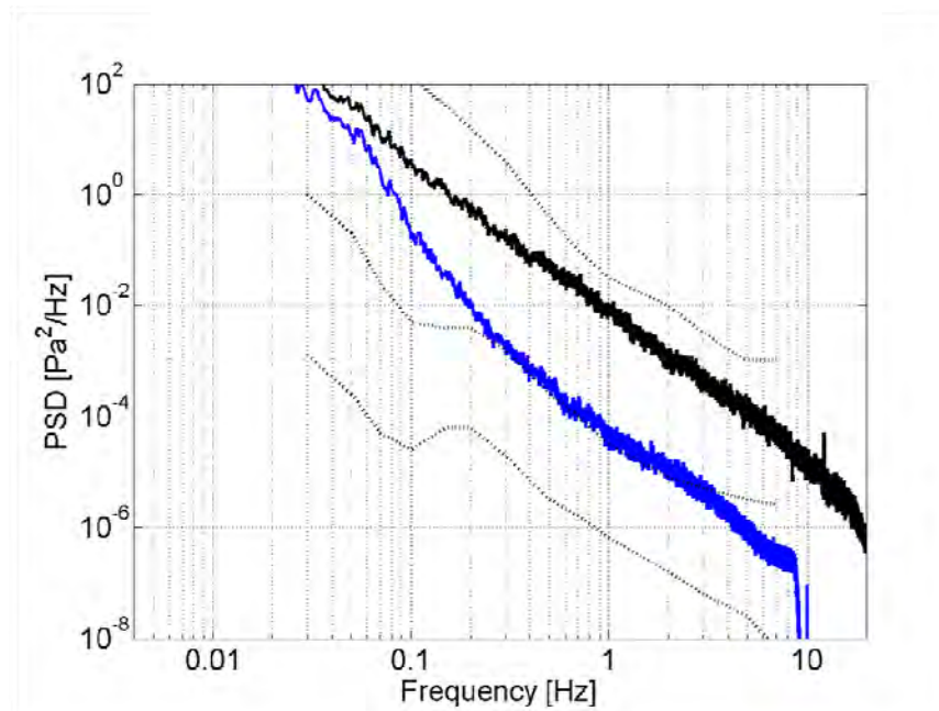
Figure 16. Pressure spectral densities for the large rosette (blue) and for the co-located reference microphone (black) for the same windy period as for Figure 15. Notice that the blue curve is lower for the large rosette than for the small rosette in the region where it parallels the single-microphone spectrum. Further, notice that the blue curve approaches the black curve at a lower frequency than for the small rosette.
