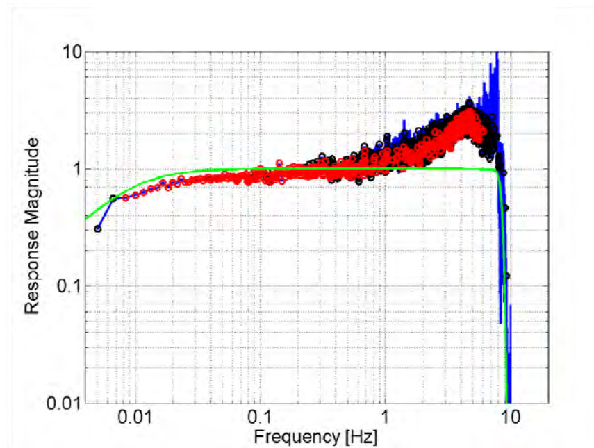
Figure 10. Magnitude response calculation for the small rosette element (V1-BFH). The calculation represents a 50-minute period starting at Day 145 01:42 UTC. The reference channel is Microphone 4. For this element, the magnitude response shows an increase at the high-frequency end that is characteristic of a resonance in the system.
