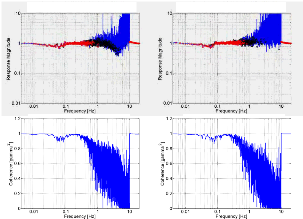
Figure 17. Magnitude response reconstructions for the larger pipe arrays using the corresponding smaller pipe array as the reference. Upper left: magnitude response of V1-BFL relative to V1-BFH; lower left: corresponding coherence; upper right: magnitude response of V2-BFL relative to V2-BFH; lower right: corresponding coherence. (The high coherence above 10 Hz is an artifact introduced by the up-sampling of the original data.)
