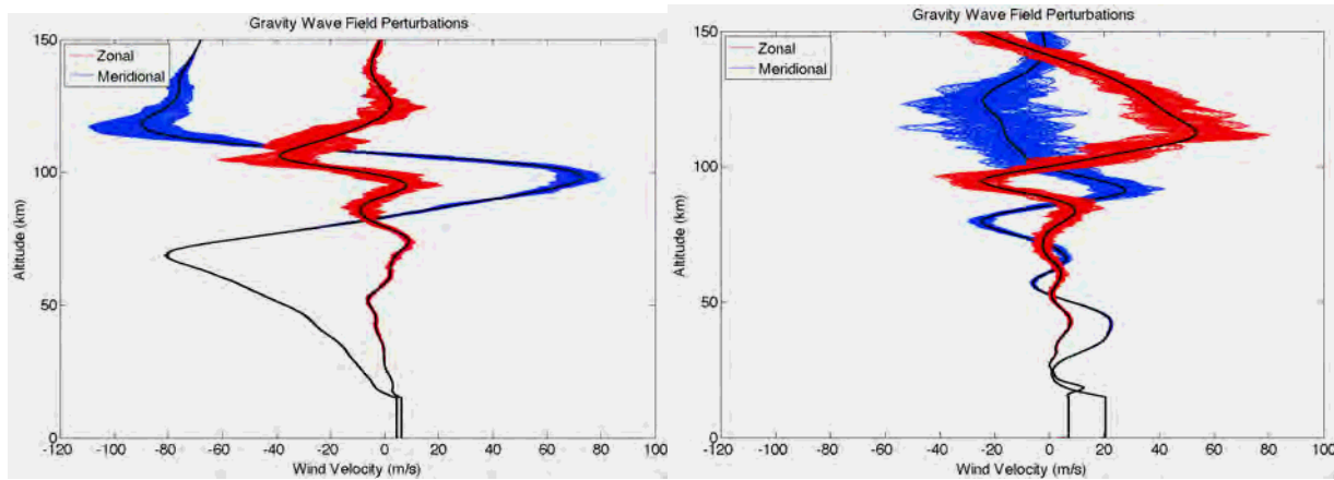
Figure 1. Zonal and meridional wind profiles, including gravity wave perturbations, for two scenarios: the Ghislenghien, Belgium event [50.6566 N, 3.879 E], which occurred on 07/30/2004 at approximately 07:00 UT (left panel); and the Gerdec, Albania event [41.394 N, 19.655 E], which occurred on 04/15/2008 at approximately 11:00 UT (right panel).
