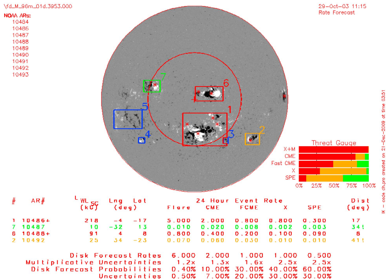
Figure 5. Sample output of the new forecast tool for 29 October 2003 (an extremely active day of Cycle 23).
