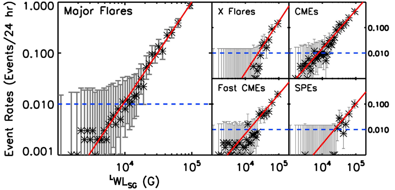
Figure 2. Log-log plots of event rates versus the free-magnetic-energy proxy. Each bin value (asterisks), its rate uncertainty ( \ell ), and the power law fits (red lines) are shown. Blue dashed lines are 0.01 events per 24 h threshold used in the fits (see text).
