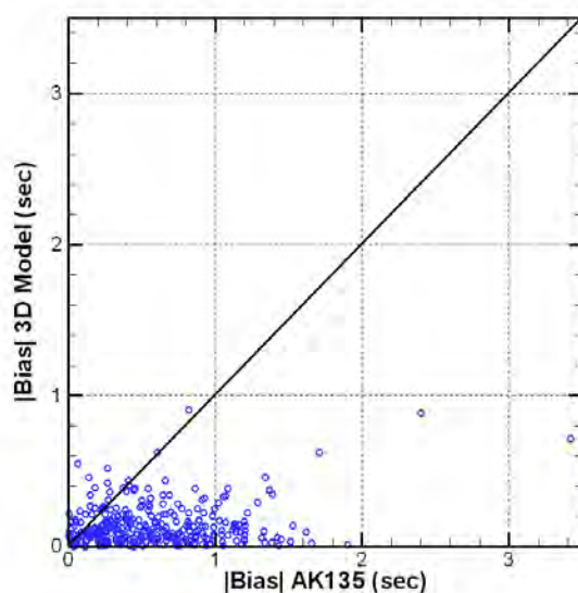
Figure 7. Median absolute value of residual computed with AK135 vs the same value computed with SALSA3D. Each point represents a single station-region pair.
