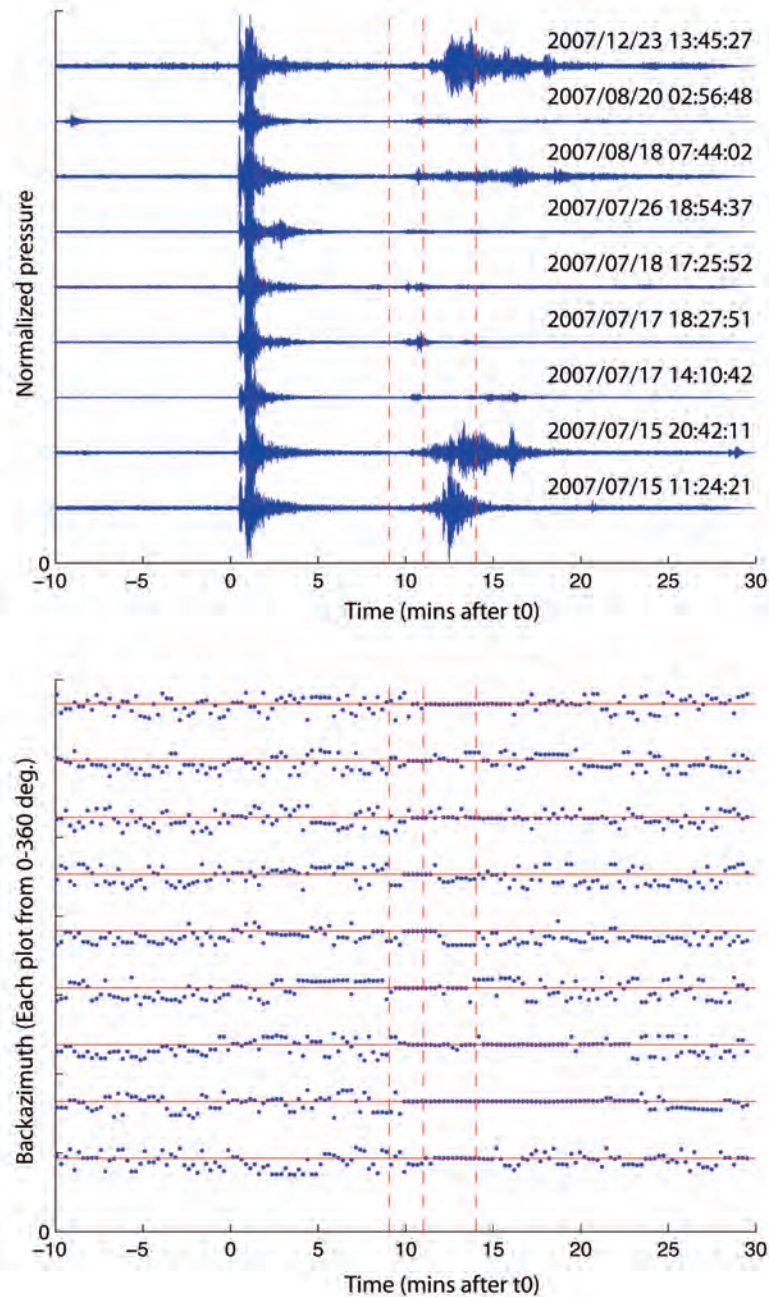
Figure 4. Detailed plot showing the waveforms associated with detected earthquakes in Tanzania (top) and corresponding derived backazimuths, with great-circle backazimuths shown by horizontal red lines (bottom). Measurements of all earthquakes in this sequence are provided in Table 1. Dashed red lines (vertical) indicate group velocities of 0.34, 0.28, and 0.22 km/s, assuming the source of infrasound corresponds to the origin time.
