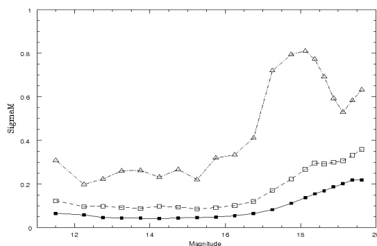
Fig. 5. 50% (■), 68% (□), and 95% (Δ) contours of the observed magnitude repeatability error as a function of mean magnitude from MJD = 56016.
