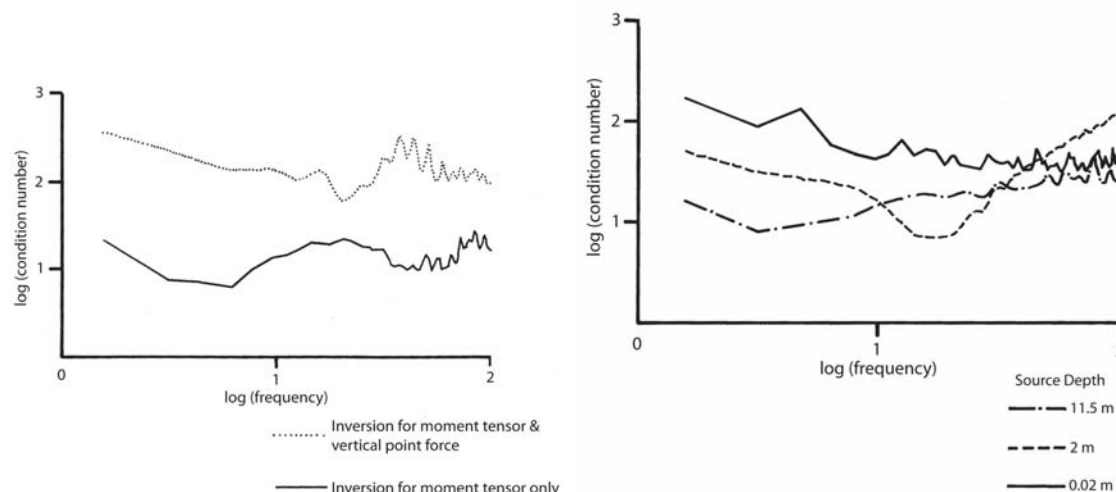
Figure 3. (Left) Condition numbers from a synthetic inversion that includes a moment tensor plus vertical point source representation and an inversion that is represented by only a moment tensors. (Right) Condition numbers for moment tensor inversions with source depths from 11.5 to 0.02 m.
