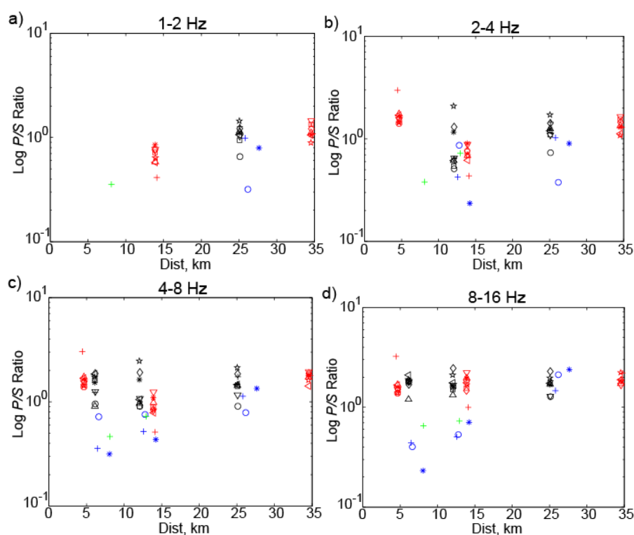
Figure 9. P/S spectral ratio as a function of distance for SPE planned and production shots. a) 1-2 Hz, b) 2-4 Hz, c) 4-8 Hz, d) 8-16 Hz. Figure key is shown in Tables 2 and 3, except blue symbols are Morenci production shots and green symbols are Black Mesa production shots.
