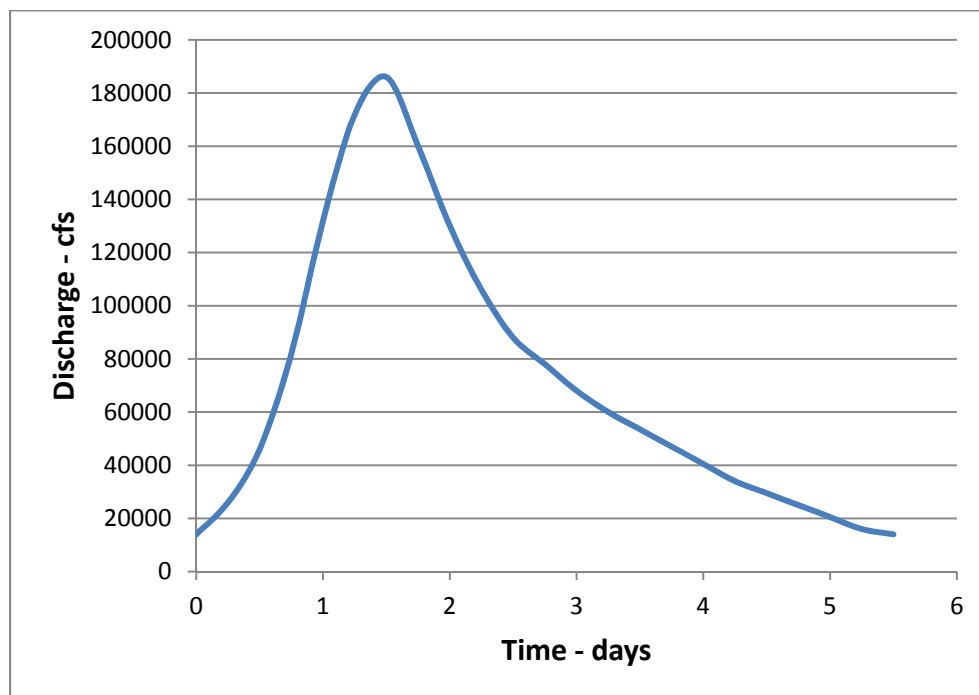
Figure 3. PMF hydrograph.
