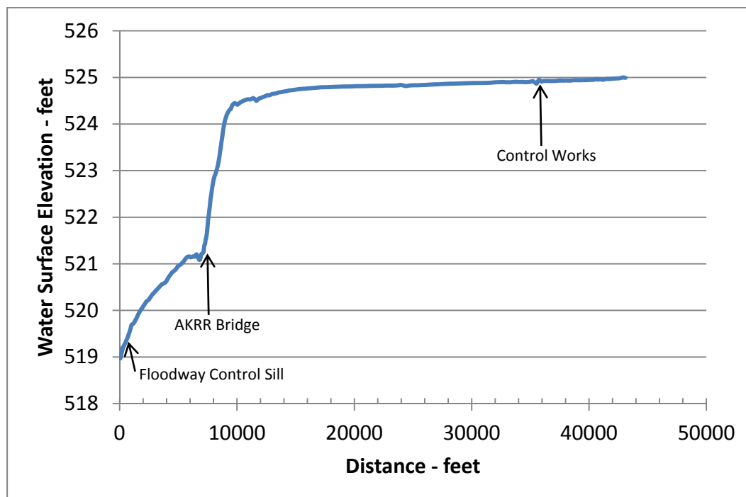
Figure 12. Longitudinal water surface profile at the peak of the PMF event – post-2010.
