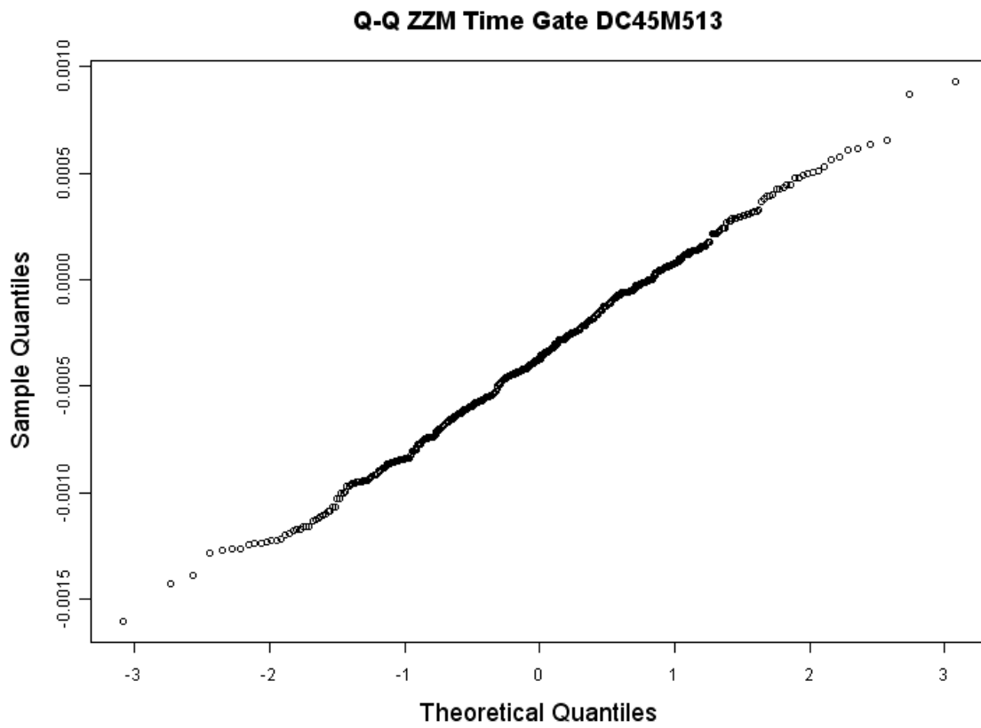
Figure 7.24. Quantile-Quantile plot of the ZMZ noise. The linearity of the line is strong evidence of gaussianity.
