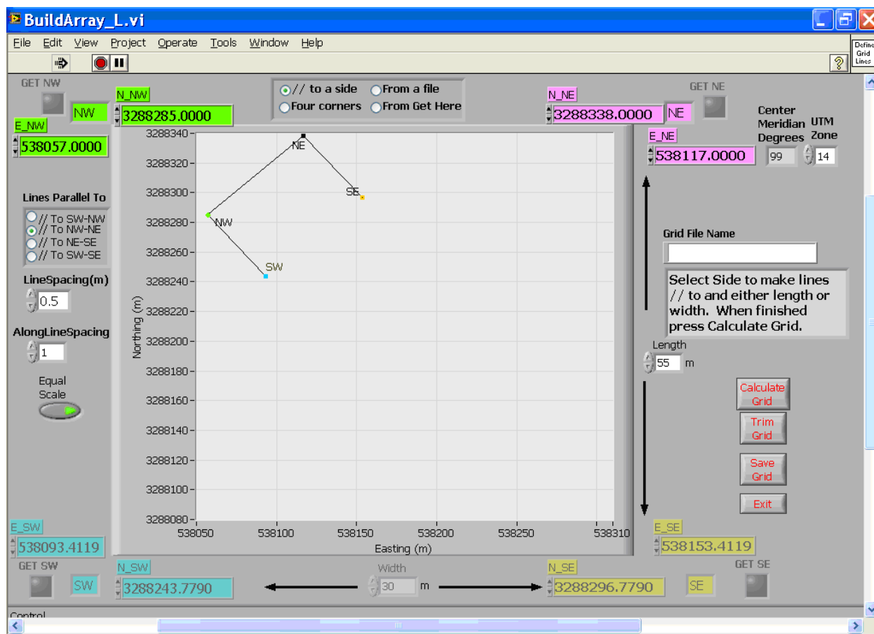
Figure 3.21. Grid planning screen, with option: // to a side, and // To NW-SW, Length = 55 m.
