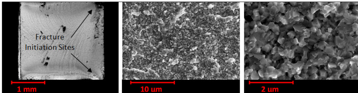
Figure 7. Fracture surface of nW SHB test specimens
