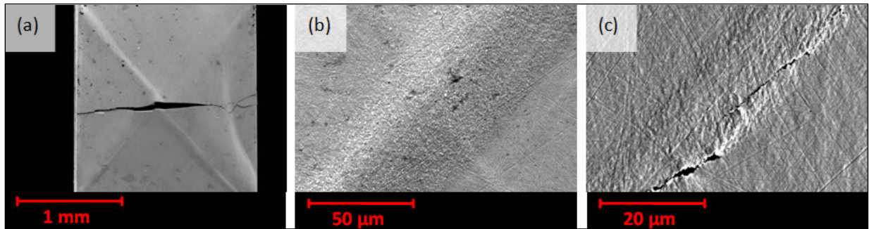
Figure 13. Surface of nW-5Re SHB compression test samples post mortem. (a) Macroscopic view of test specimen. (b) High magnification image of shear localization appearing at 45° to the loading direction. (c) High magnification image of combined shear localization and fracture failure mechanisms.
