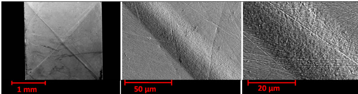
Figure 18. Post mortem images of SHB compression test samples with clear evidence of shear localization at 45° to the loading direction.
