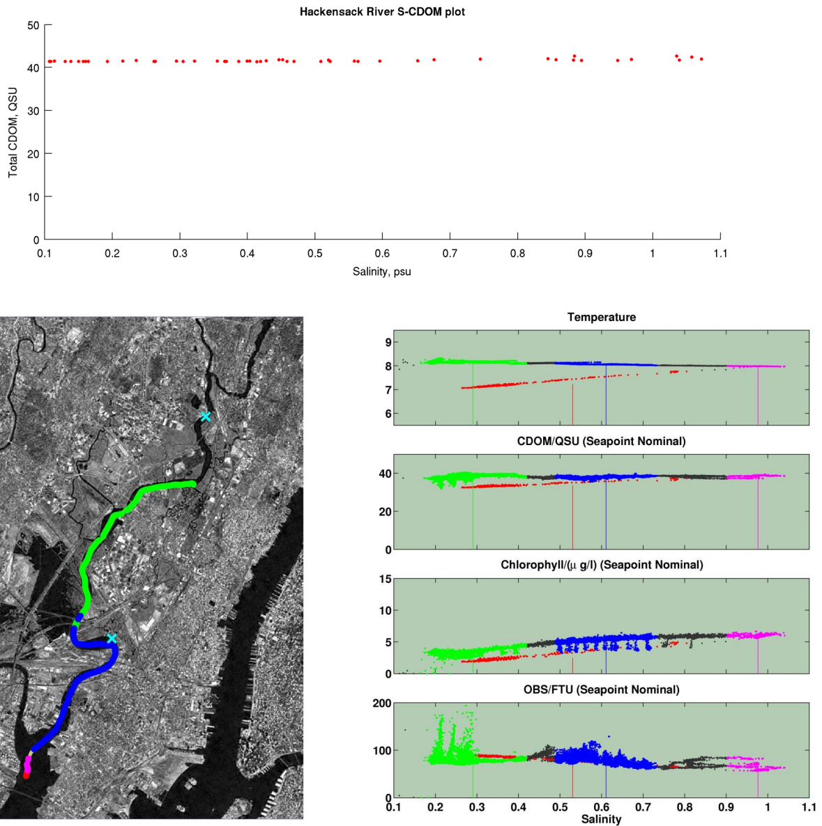
Figure 13. NYHOPS HIGHRES validation for April 17, 2007 major flooding event. Top panel shows high resolution NYHOPS CDOM model results predicted for the time observations (lower panels) were taken, between 16 and 18 hrs ET. Both model and data show that the Hackensack, influenced by historic inflows, was a freshwater river all along its span at the time that CDOM concentrations were measured. Both model and data show CDOM concentrations throughout the river close or equal 40 QSU, with an almost imperceptible slight increase at the Newark Bay outlet. Although due to tidal time logistics the observations stopped south of the Bergen County plant outfall, the CDOM load from the plant was diluted by the historic freshwater drainage inflows and cannot be discerned in the model.
