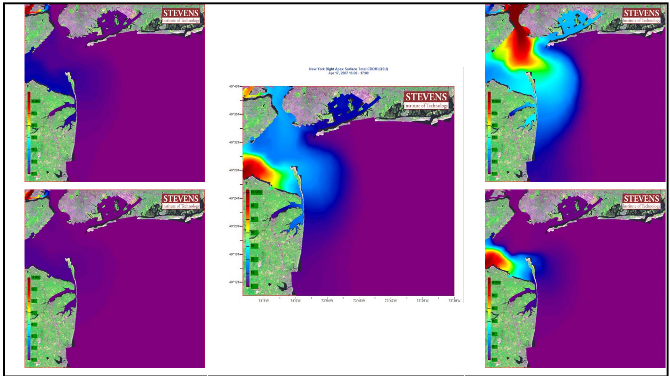
Figure 14. Screen captures of high resolution NYHOPS-predicted CDOM for April 17, 2007 16:30 ET, same time frame as in Figures 12 and 13. This date was one of major flooding all along northern New Jersey due to very intense and long-lasting rainfall. The various end members (clockwise from top left, Passaic River, Hudson River, Raritan River, and Hackensack River including the Bergen County water treatment plant), combine their strengths to create the central image which depicts the predicted CDOM concentration in the surface waters of the New York Bight Apex. Note the different scales in the end member color maps. Due to record-breaking river flows, considerable CDOM concentrations were predicted by the NYHOPS model to exit New York Harbor proper and influence the New York Bight region, hugging the northern New Jersey Atlantic shoreline carried by southbound alongshore transport.
