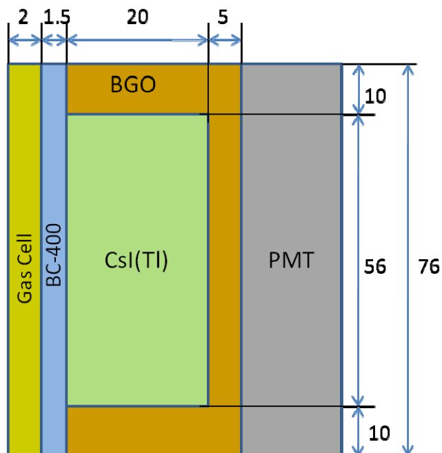
Figure 2. Schematic diagram of ASP detector designed to reduce Compton continuum in the regions of interest and shield the gamma detector against background radiation. All dimensions are in millimetres.
