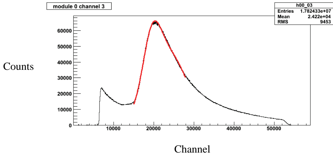
Figure 1. Muon spectrum collected with three 2"-thick plastic scintillator panels "T"ed together. These are the panels making up the active veto on the top surface of the lead shield. The lower energy threshold, as set in this figure, will accept some gamma background to ensure a high rate of muon exclusion.
