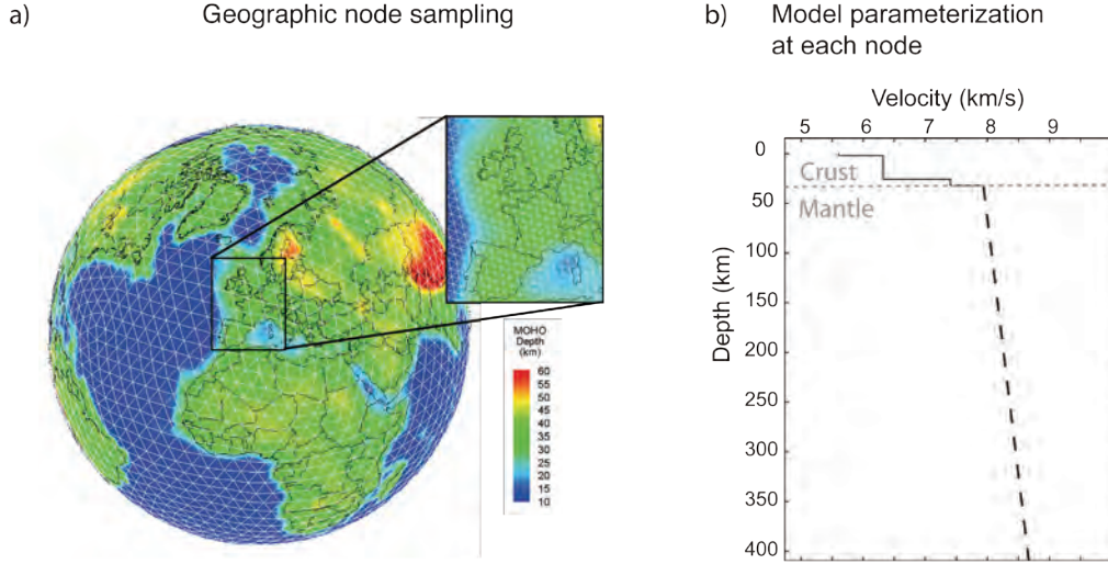
Figure 2. Global model parameterization. a) An example tessellation with approximately 5° grid spacing. The inset shows the 1° used in this study. Color indicates Moho depth of the starting model. b) An example velocity/depth profile as defined at each node. The mantle portion of the profile is specified by the velocity at the crust/mantle interface and a linear gradient. (Reproduced from Myers et al., 2010)
