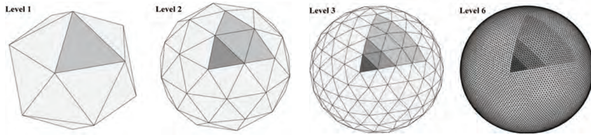
Figure 1. Spherical tessellation grids and parent-daughter triangle relationships. The initial object (a regular icosahedron; Level 1) consists of 20 triangular faces and 12 distinct vertices. The triangular faces (parents) are recursively subdivided into smaller triangles (daughters) and the vertices are normalized to the unit sphere. Each recursion represents a level in the tessellation hierarchy and parent-daughter triangle relationships are indexed for efficient communication. Triangular regions are shaded simply for visual orientation of the parent-daughter regions and sub-regions.
