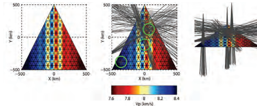
Figure 2. Synthetic tomography scenario imitating a combination of regional and teleseismic phases and complex shallow upper mantle velocity structure parameterized by a triangular tessellation with 5 hierarchical levels. (left) Synthesized velocity structure with a regional trend (from left to right) and embedded, small-scale velocity heterogeneities. (center) Map view of synthetic ray path coverage consisting of several clusters of sub-horizontal regional phase ray paths and 3 clusters of near-vertical teleseismic ray paths (highlighted with green circles). (right) 3-D view of the synthesized ray path coverage.
