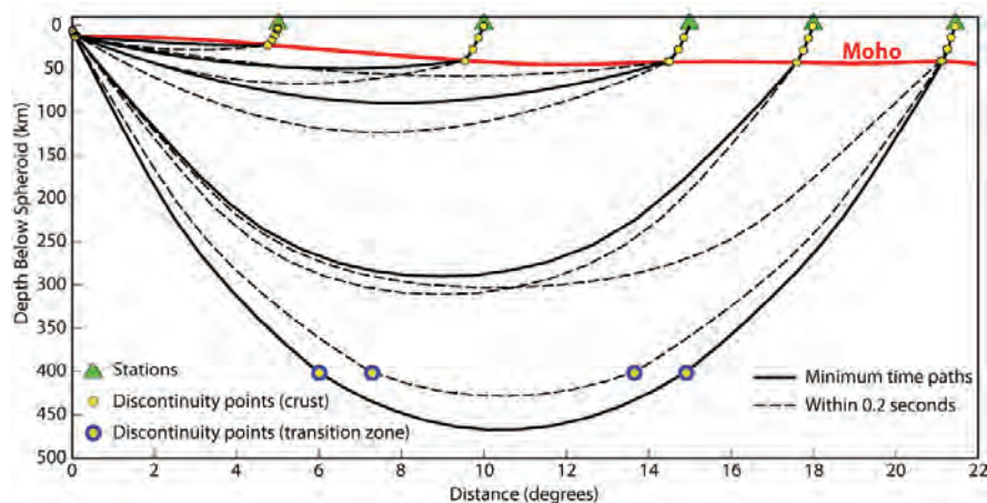
Figure 6. Example 3-D ray paths calculated through the global velocity model constructed in this study. Sensitivity is spread across broad depth zones and/or multiple model units to mitigate the problem of interdependence of paths and velocity structure as well as multi-pathing.
