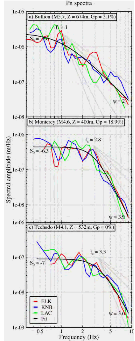
Figure 3. P_n spectra examples with the name, magnitude (where M = m_b[P_n] ), depth ( Z ), and gas porosity ( G_p ) given in the subtitles. The long-period level ( S_0 ), corner-frequency ( f_c ), and fall-off ( \psi ) are given in each plot, and the spectra are colored by station and the fit is shown in the legend in the lowermost plot. a) Spectra for an event with low G_p and \omega^{-2} fall-off. b) Spectra for an event with high G_p and high fall-off. c) Spectra for an event with low G_p and high fall-off.
