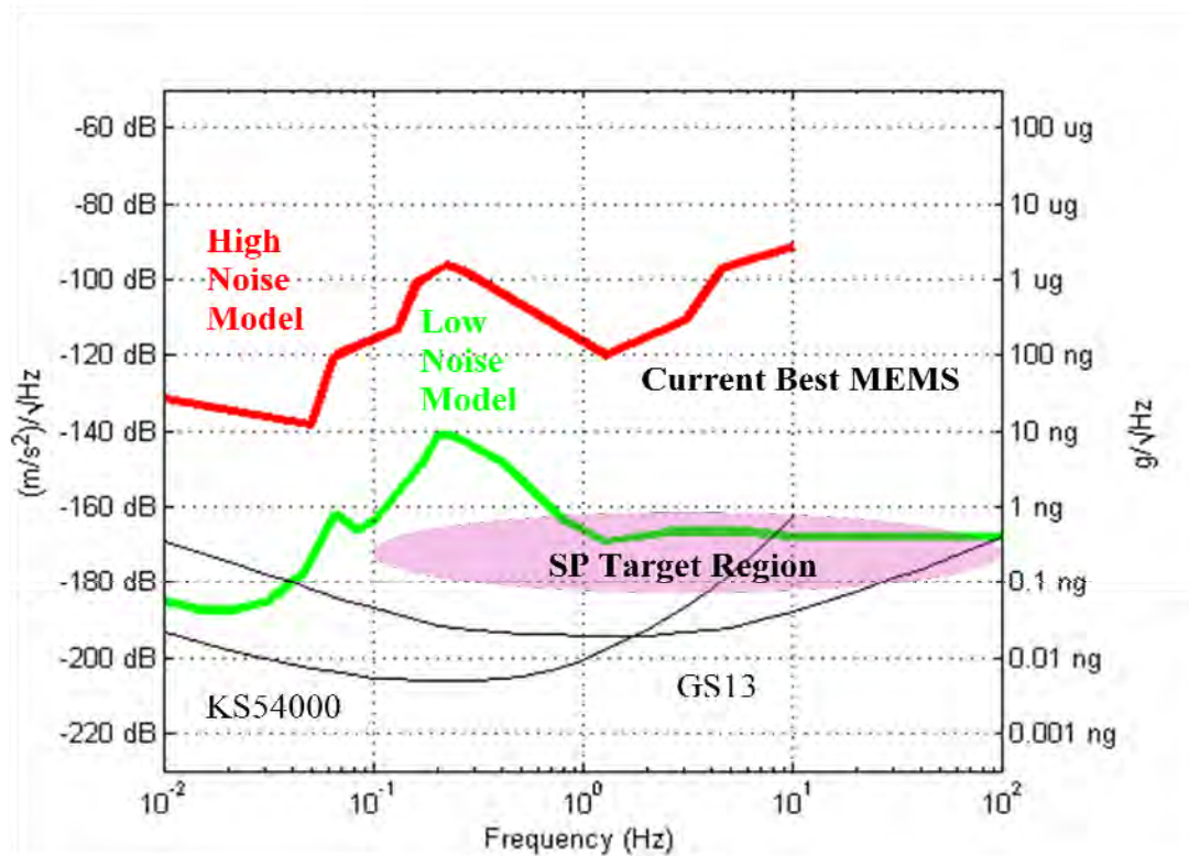
Figure 5. Seismometer R&D is directed and constrained by Earth noise. USGS High Noise (red) and Low Noise (green) models are shown with current capabilities and future targets.
