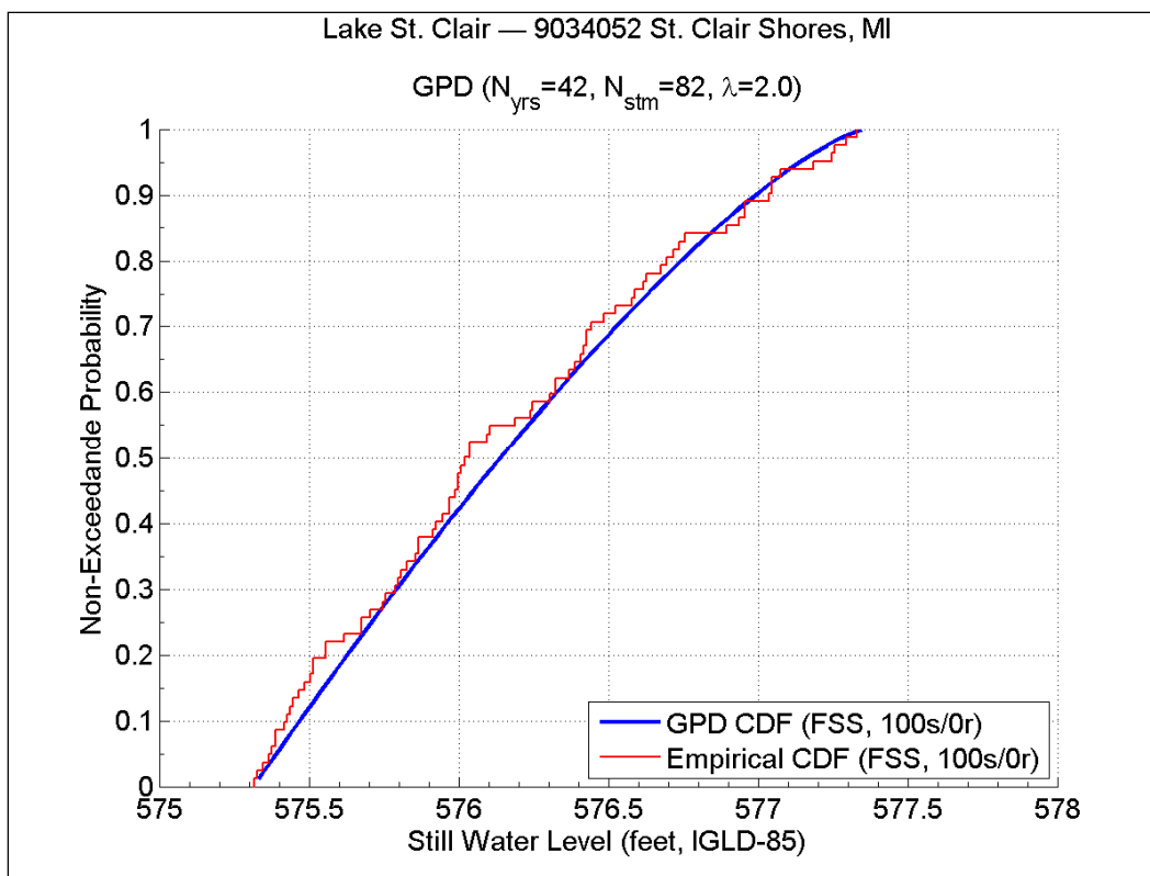
Figure D7. SWL CDF plot from FSS (with convective storms) for St. Clair Shores, MI.
