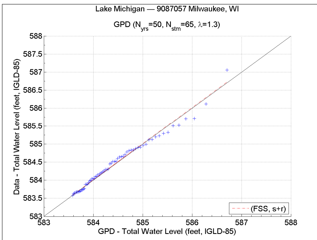
Figure A13. TWL Q-Q plot from FSS (s+r, with convective storms) for Milwaukee, WI.
