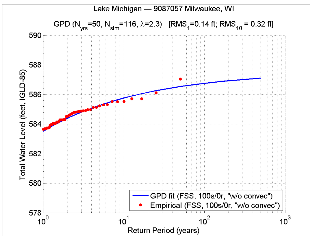
Figure 71. TWL RP plot from FSS (100s/0r, no convective storms) for Milwaukee, WI.
