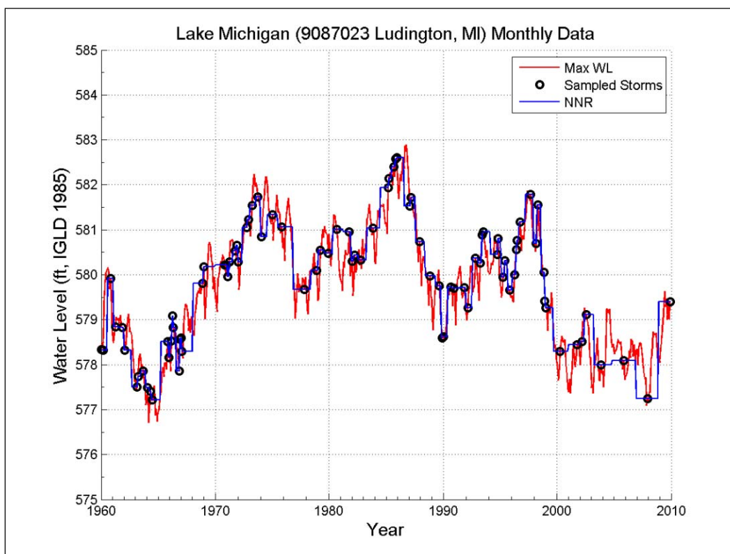
Figure 28. Distribution of 100-storm CSS across lake levels for Ludington, MI.
