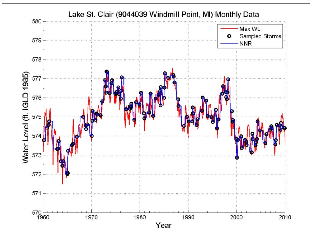
Figure D5. Distribution of 150-storm CSS across lake levels for Windmill Point, MI.
