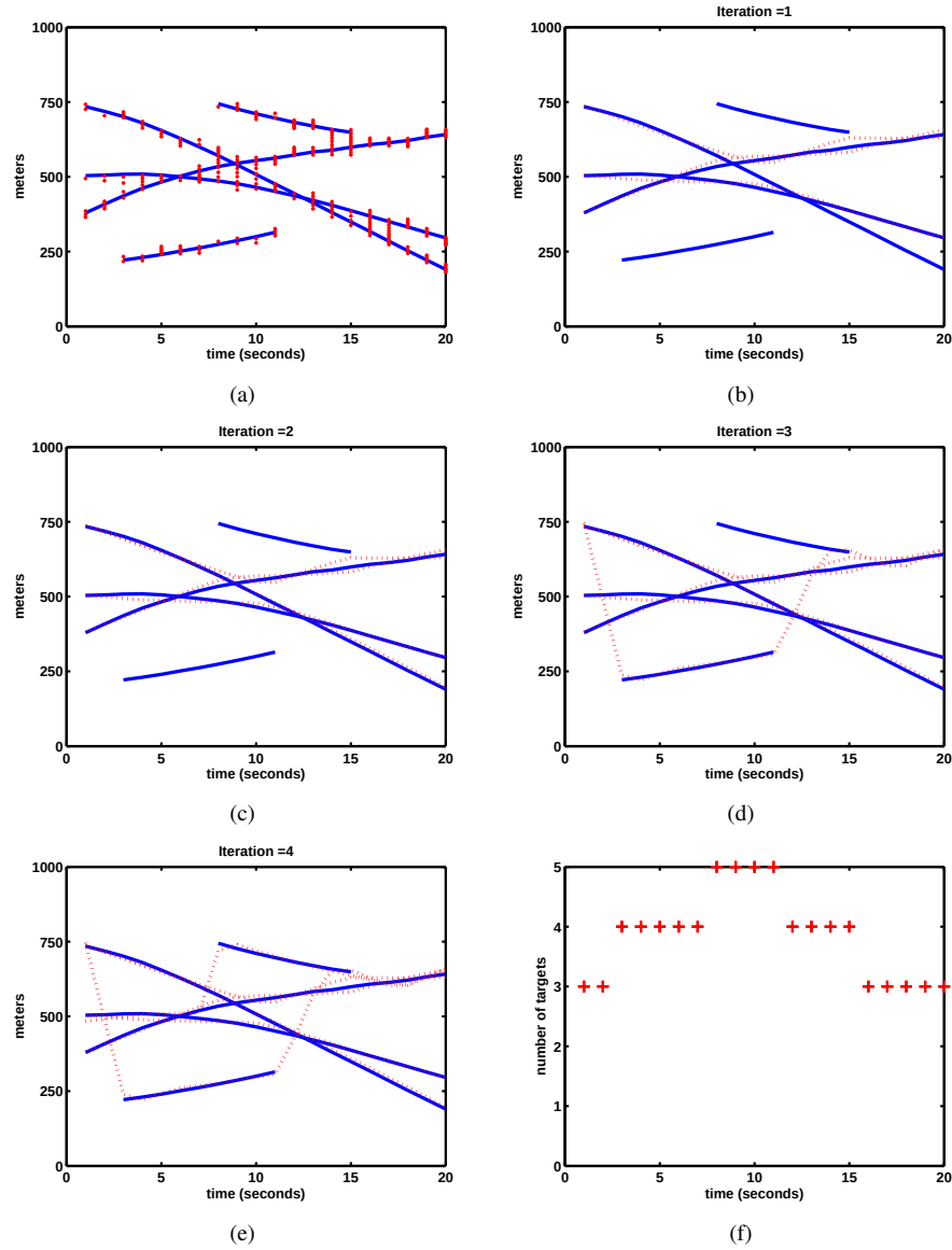
Fig. 16. For target birth/death cases, (a). estimated target positions using PHD vs. time (b)-(e). at each iteration of ClusterTrack, positions of cluster heads vs. time, where true target tracks are in solid lines, and dots or dashed lines denote the estimates using either PHD or ClusterTrack method, respectively. (f). the number of targets versus time
