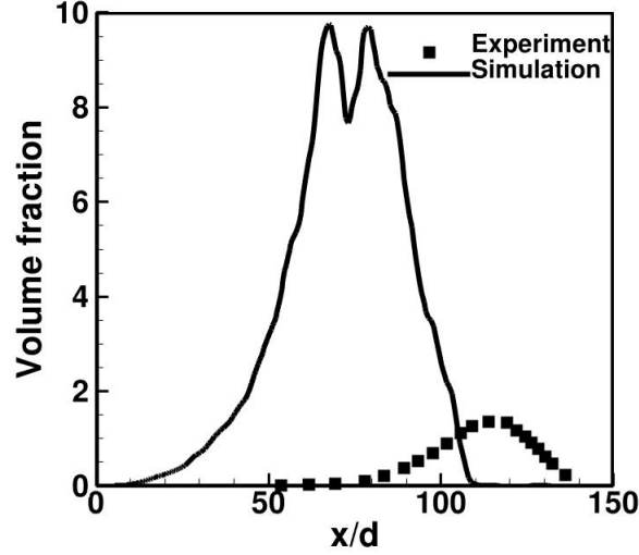
Figure 49: Comparison of soot volume fraction from the simulation with the experiment of Qamar, et. al. [3]. The data is plotted along the centerline.
