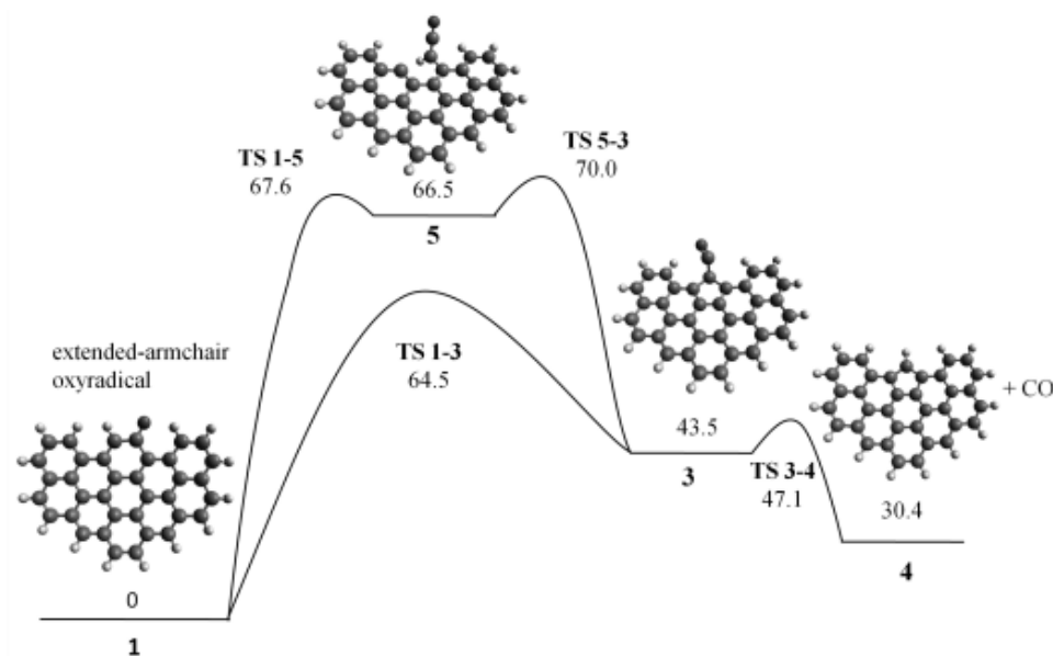
Figure 23: Minimum potential energy paths for the thermal decomposition of the extended-armchair oxyradical at the B3LYP/6-311G(d,p) level. Energies are in kcal/mol at 0 K relative to the reactant.
