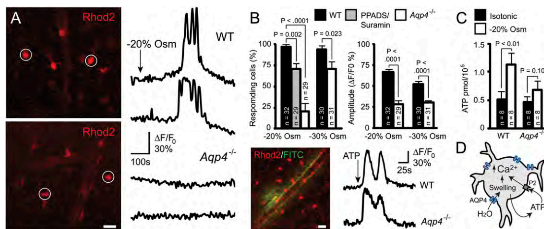
Fig. 3. Osmotically induced astrocytic \text{Ca}^{2+} responses and ATP release in vitro. (A) Two-photon images of Rhod2 AM-loaded acute cortical slices obtained from WT (Upper) and \text{Aqp4}^{-/-} (Lower) mice. Traces shown are from astrocytes marked in Left. Exposure of slices from WT mice to aCSF with 20% reduction in osmolarity ( -20\% Osm) induced brisk astrocytic \text{Ca}^{2+} spikes. In contrast, this osmotic stress failed to elicit \text{Ca}^{2+} spikes in most AQP4-deficient astrocytes. (B) Quantitative analysis of astrocytic \text{Ca}^{2+} responses to osmotic stress. Deletion of \text{Aqp4} or blocking P2 purinergic receptors with PPADS/suramin significantly reduced the number of astrocytes that responded with \text{Ca}^{2+} spikes during exposure to -20\% Osm. When more severe hypoosmotic stress ( -30\% Osm) was applied, a larger fraction of the \text{Aqp4}^{-/-} astrocytes responded. The amplitude of the \text{Ca}^{2+} spikes differed between the genotypes for both types of stress. Image shows intense \text{Ca}^{2+} signals in Rhod2-loaded astrocytes after microinjection of ATP and FITC-dextran (green; to verify injection) into the slice. Representative traces from WT and \text{Aqp4}^{-/-} mice are shown. (C) Cultured astrocytes exposed to hypoosmotic media ( -20\% Osm, 15 min) released significantly more ATP than those kept in isotonic media. Astrocytes from \text{Aqp4}^{-/-} mice did not show osmotically induced ATP release. P values were obtained by two-tailed Student t test. Error bars represent SEM. (Scale bar: 25\ \mu\text{m} .) (D) Diagram showing proposed involvement of AQP4 in astrocyte signaling cascades during hypoosmotic stress. AQP4-mediated water influx triggers \text{Ca}^{2+} transients, partly by promoting release of ATP and activation of P2 purinergic receptors.
