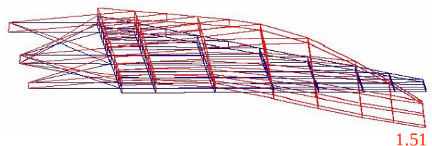
Figure 10. Mach 0.85 deformation
