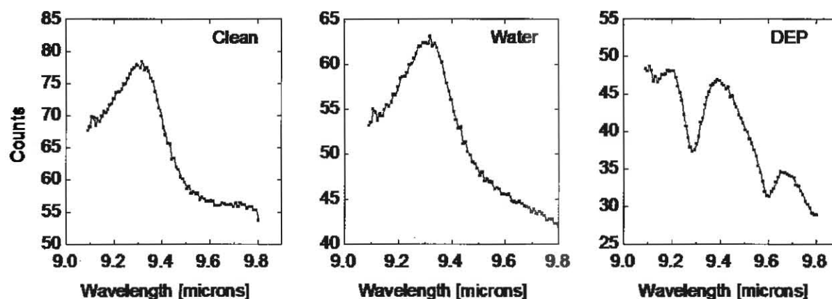
Figure 5: Spectral reflectance from clean concrete pavers (left), concrete with water (center), and concrete with DEP (right).
