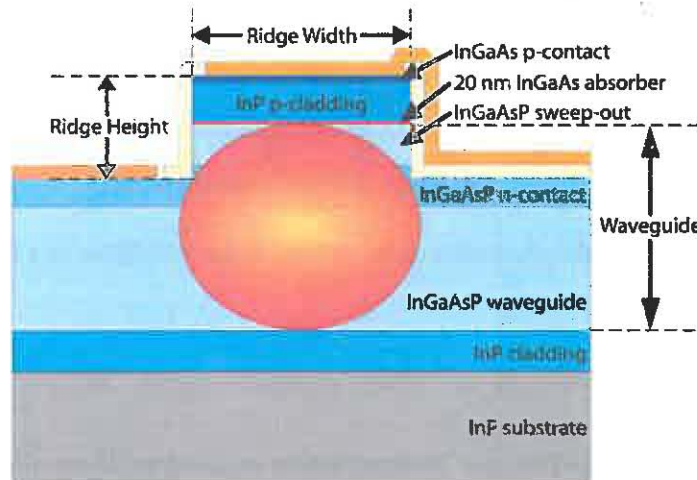
Fig. 2. Cross-section of the SCOWPD, showing the fundamental mode location and overlap with the InGaAs absorber, ridge height ( 2.75\text{ }\mu\text{m} ), ridge width, and thick waveguide ( 5\text{ }\mu\text{m} ).
